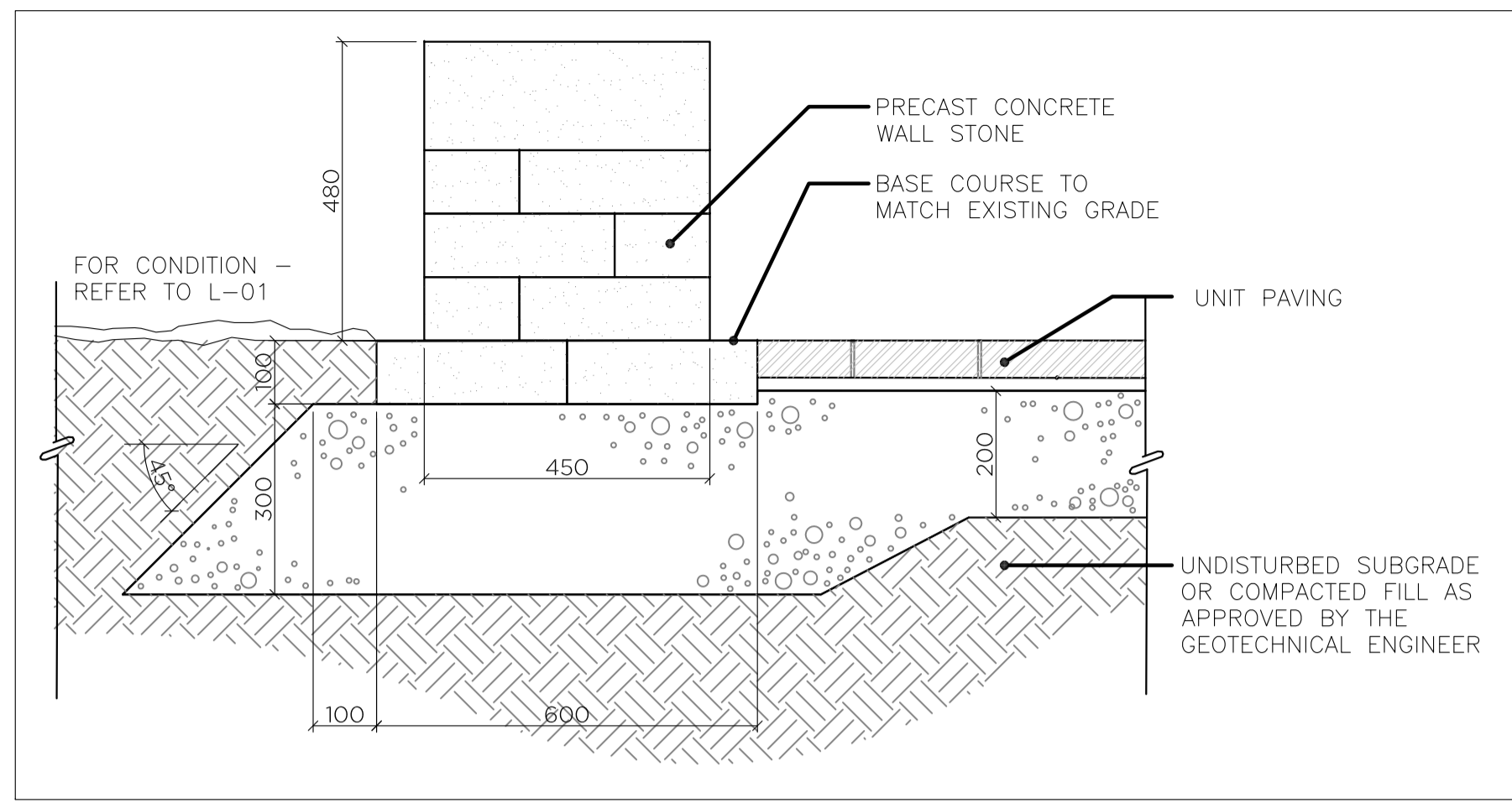
1 FREESTANDING SEATING WALL N.T.S. L-02
