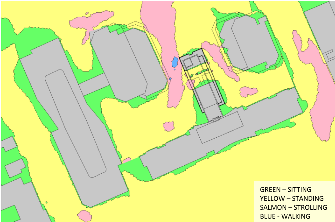
FIGURE 3: SPRING – GRADE-LEVEL PEDESTRIAN WIND CONDITIONS
