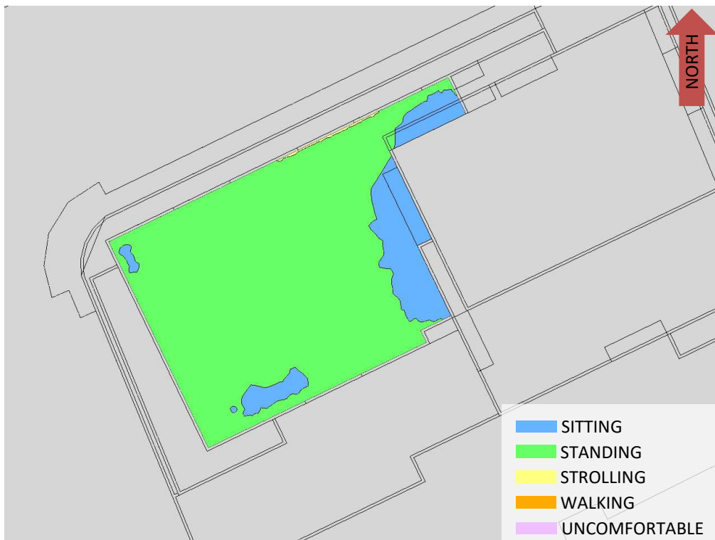
FIGURE 7B: SUMMER – WIND COMFORT, LEVEL 7 COMMON AMENITY TERRACE
