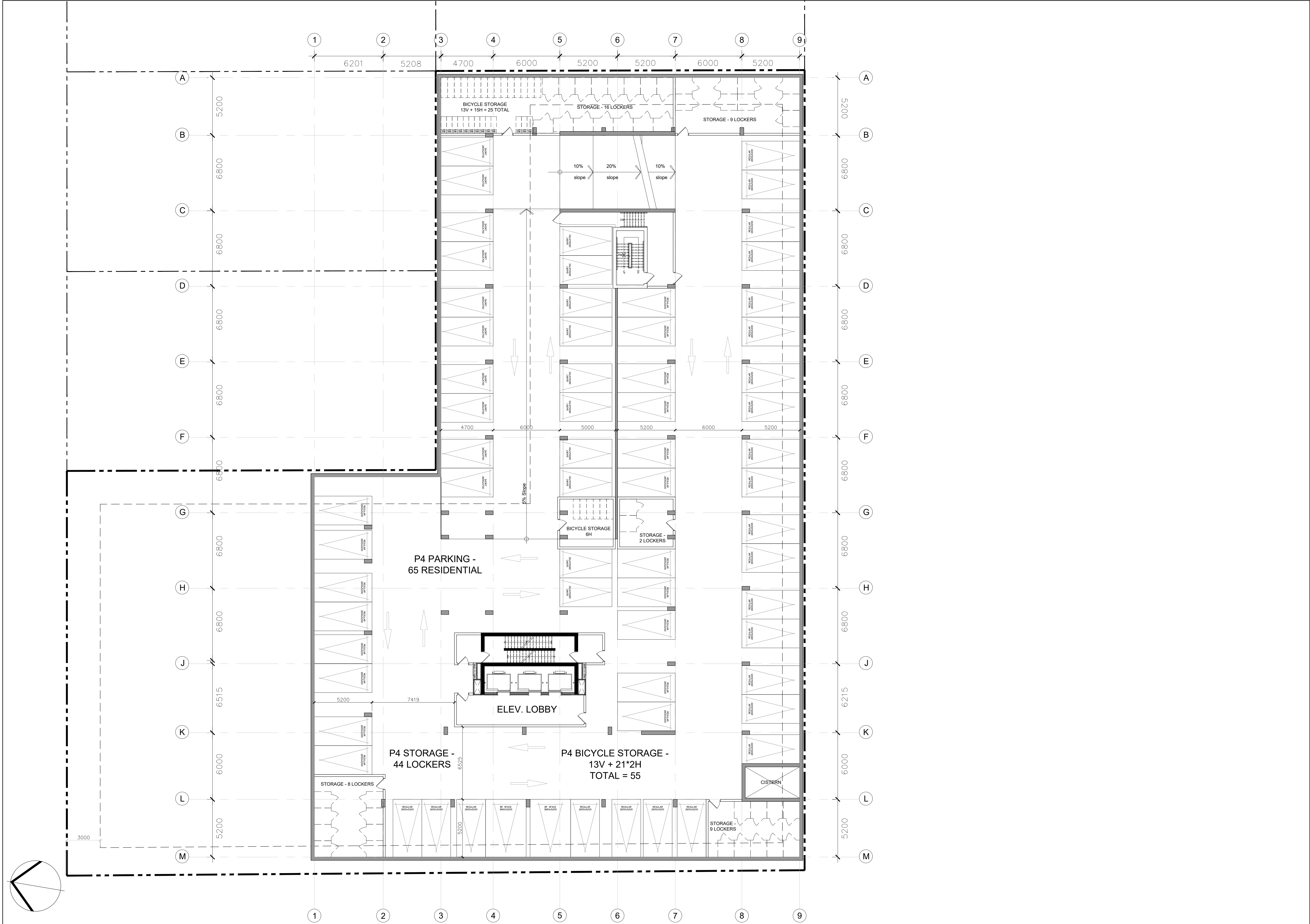
1 LEVEL P4 FLOOR PLAN A2.04 1:150
