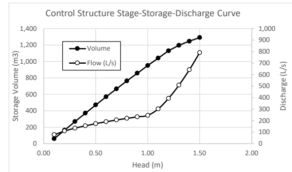
Stage-Storage-Discharge Curve for Control Structure
