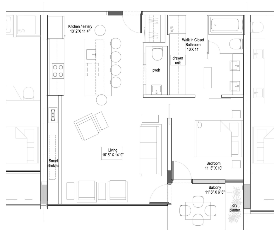
1 Bedroom 1 & 1/2 Bath 635 s.f.
