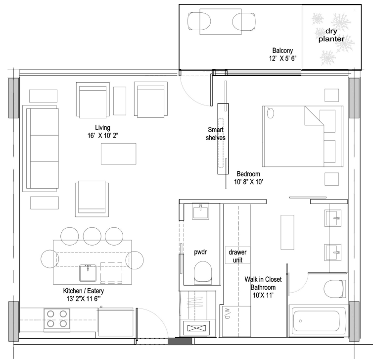
1 Bedroom 1 & 1/2 Bath 580 s.f.
