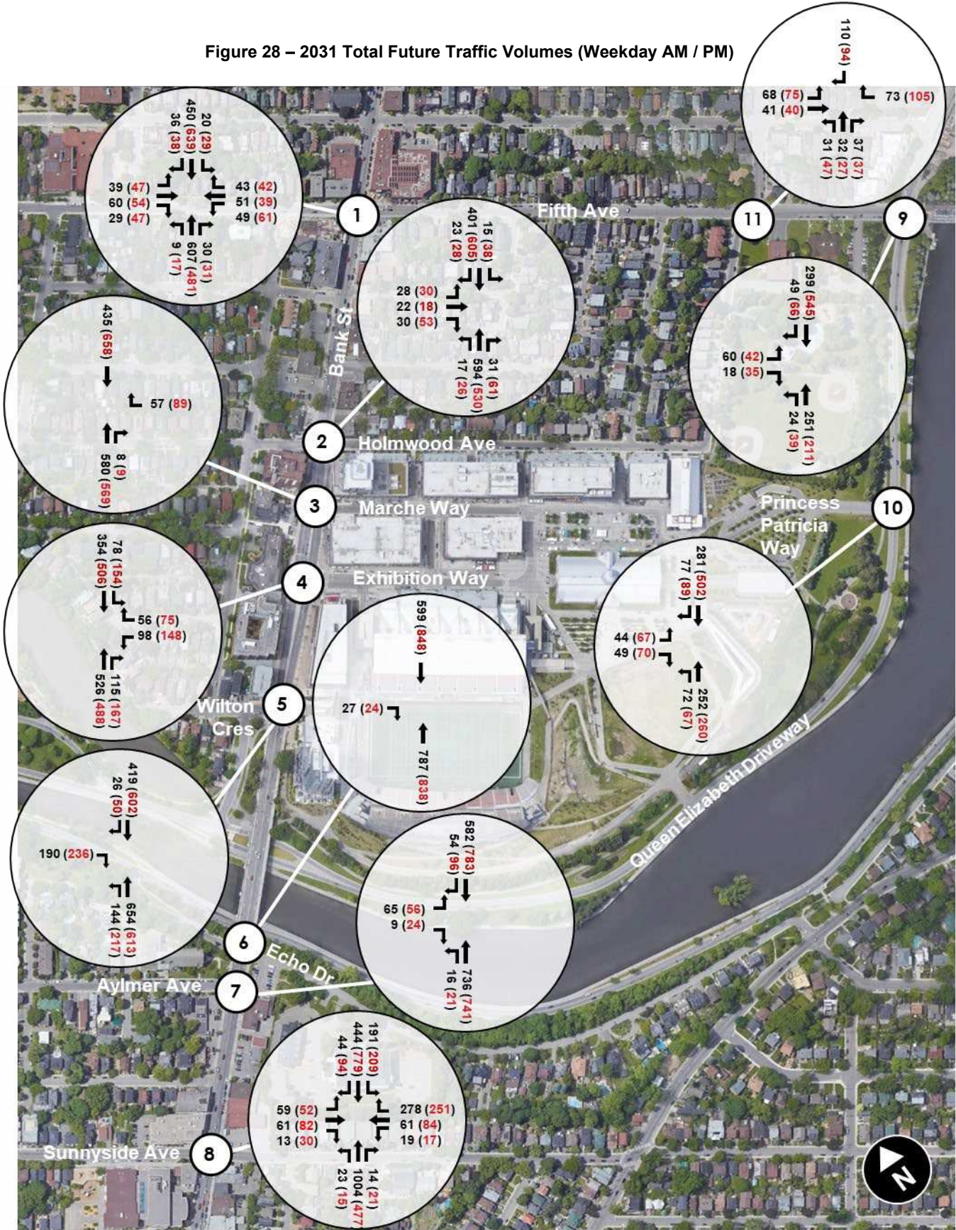
2031 Total Future Traffic Volumes (Weekday AM and PM Peak Hour) AM Peak Hour (PM Peak Hour)
