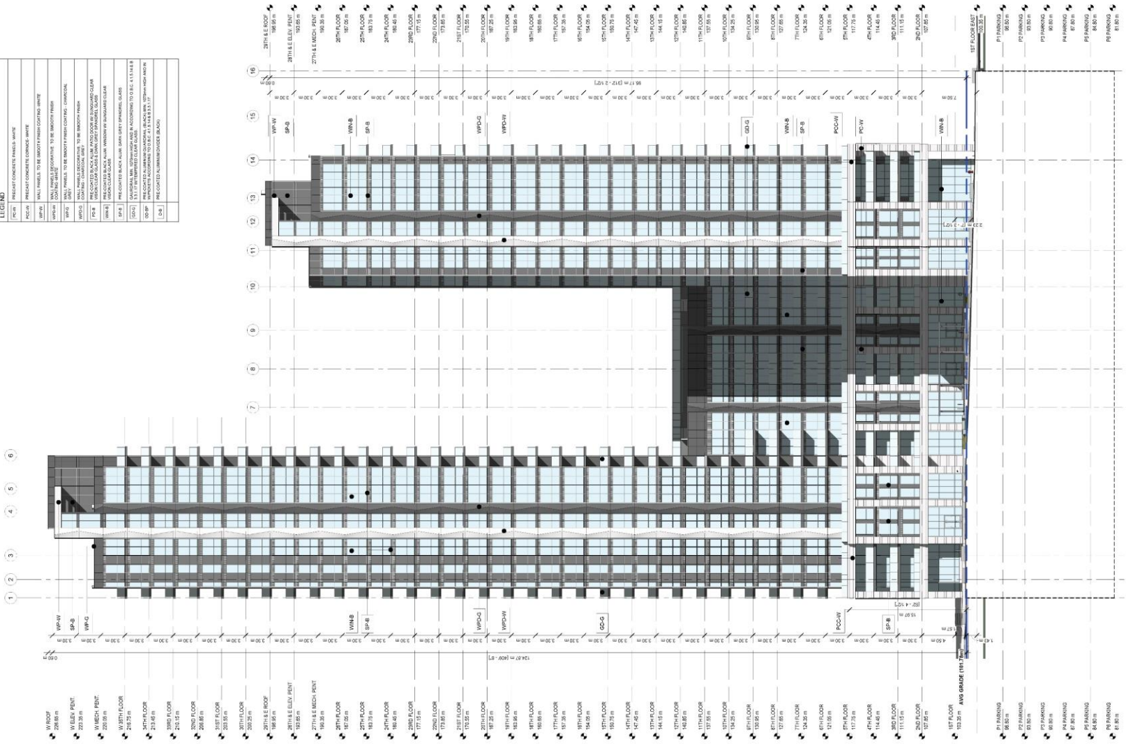
SOUTH ELEVATION 1 : 200
