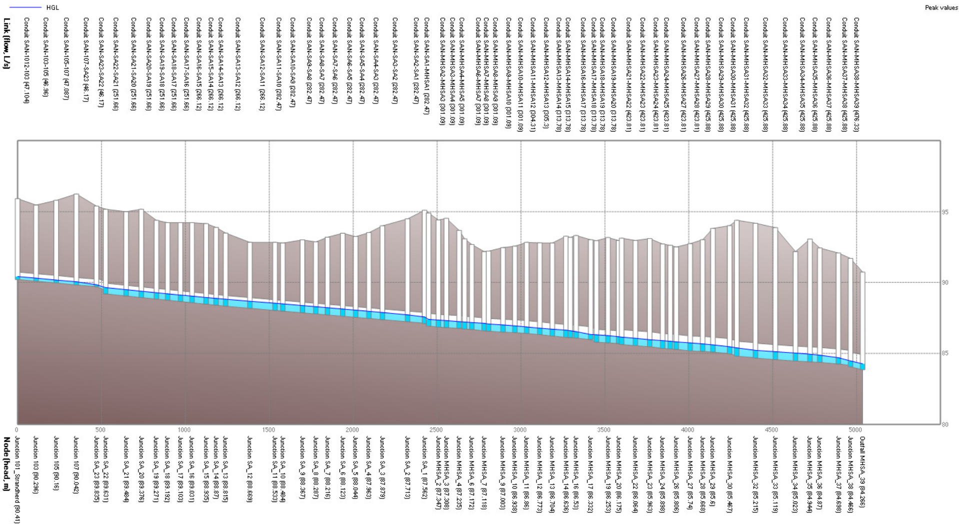
Figure 2 - Existing Conditions HGL Profile
