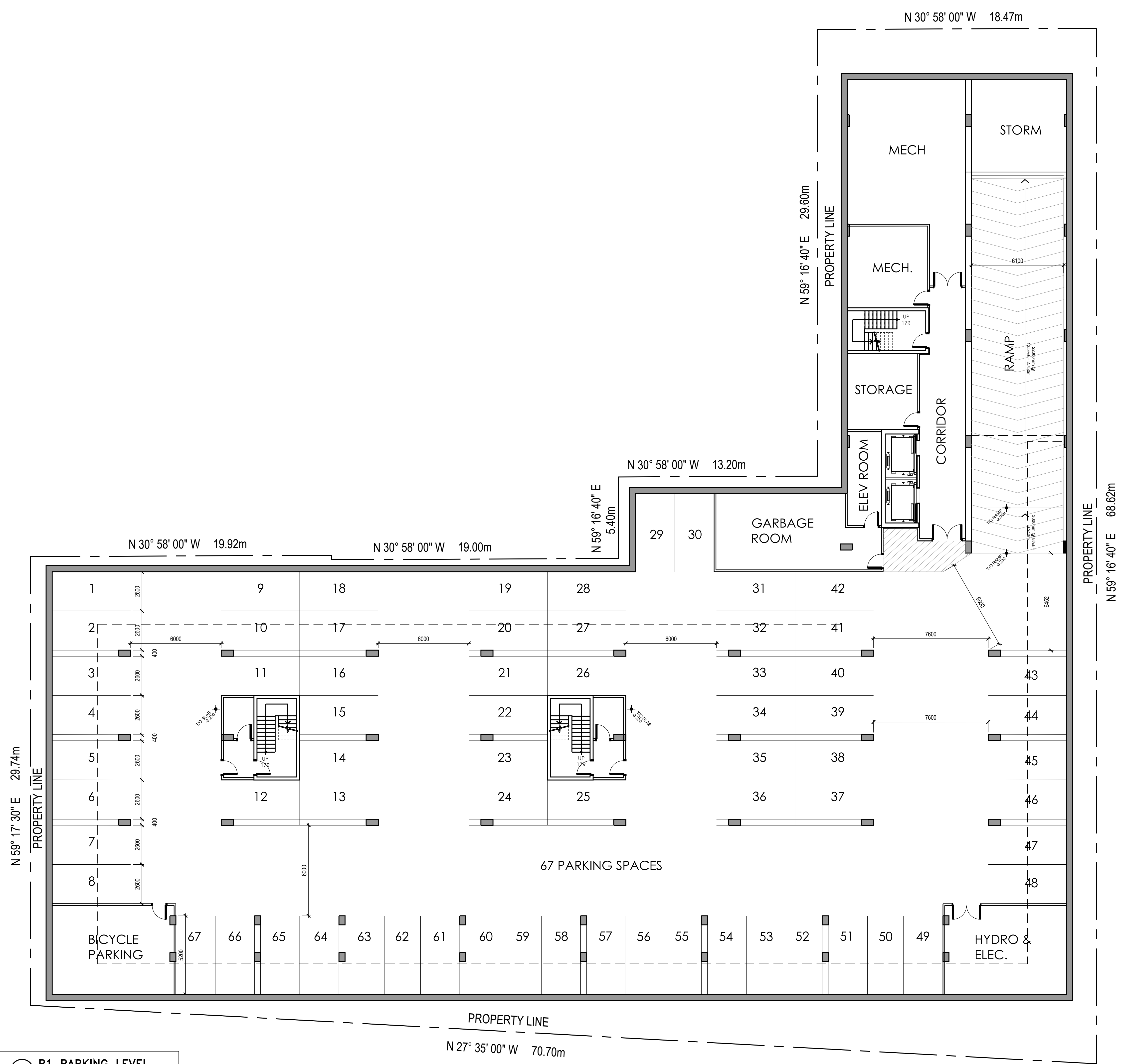
1 P1 PARKING LEVEL SCALE 1:125
