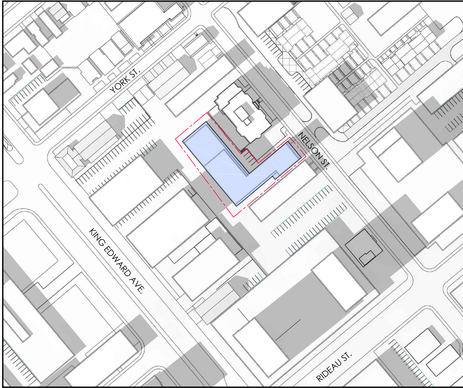
SEPTEMBER 21 - 12PM
