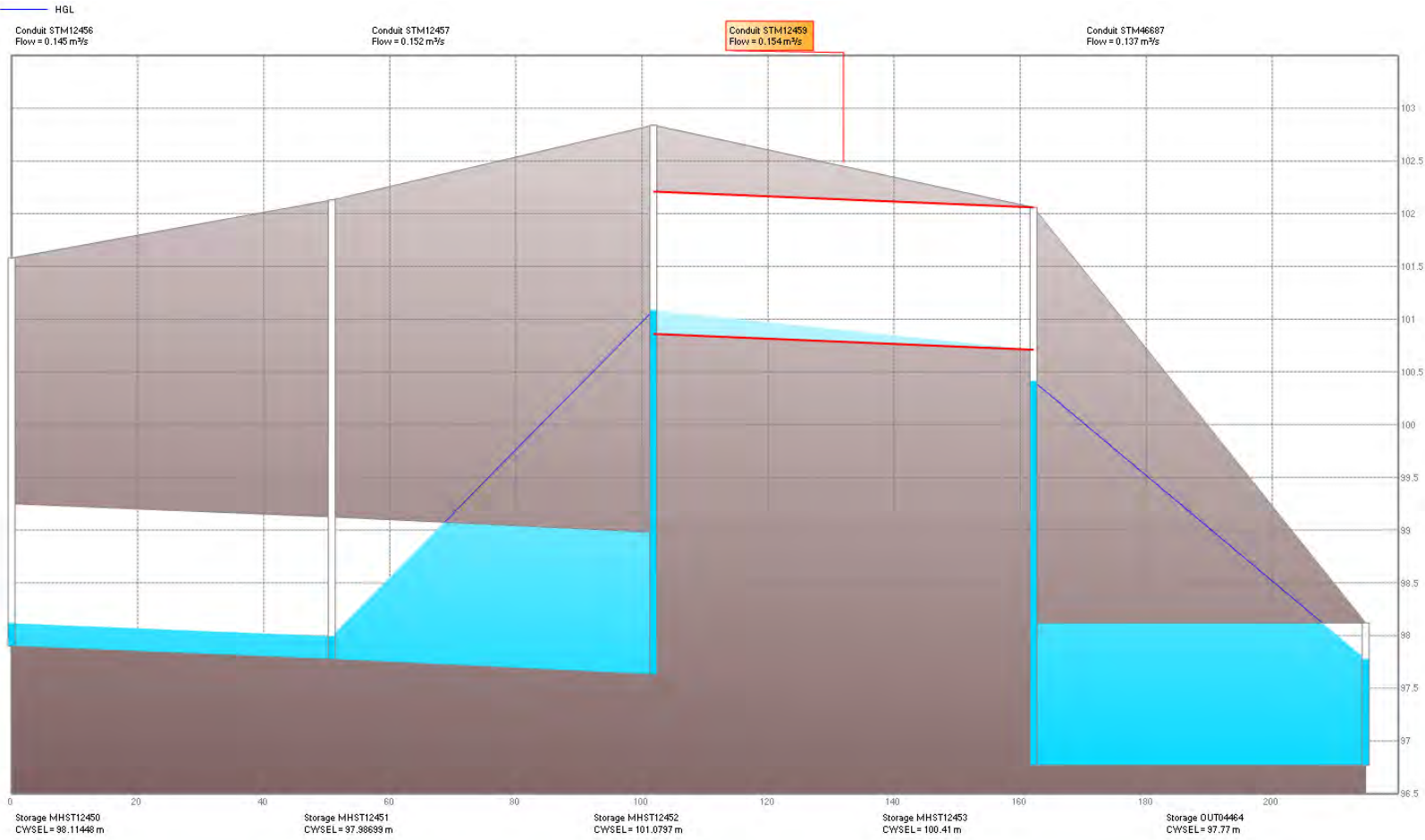
Figure A5: STM12459 – Link inlet and outlet elevations do not match neighbouring pipes
