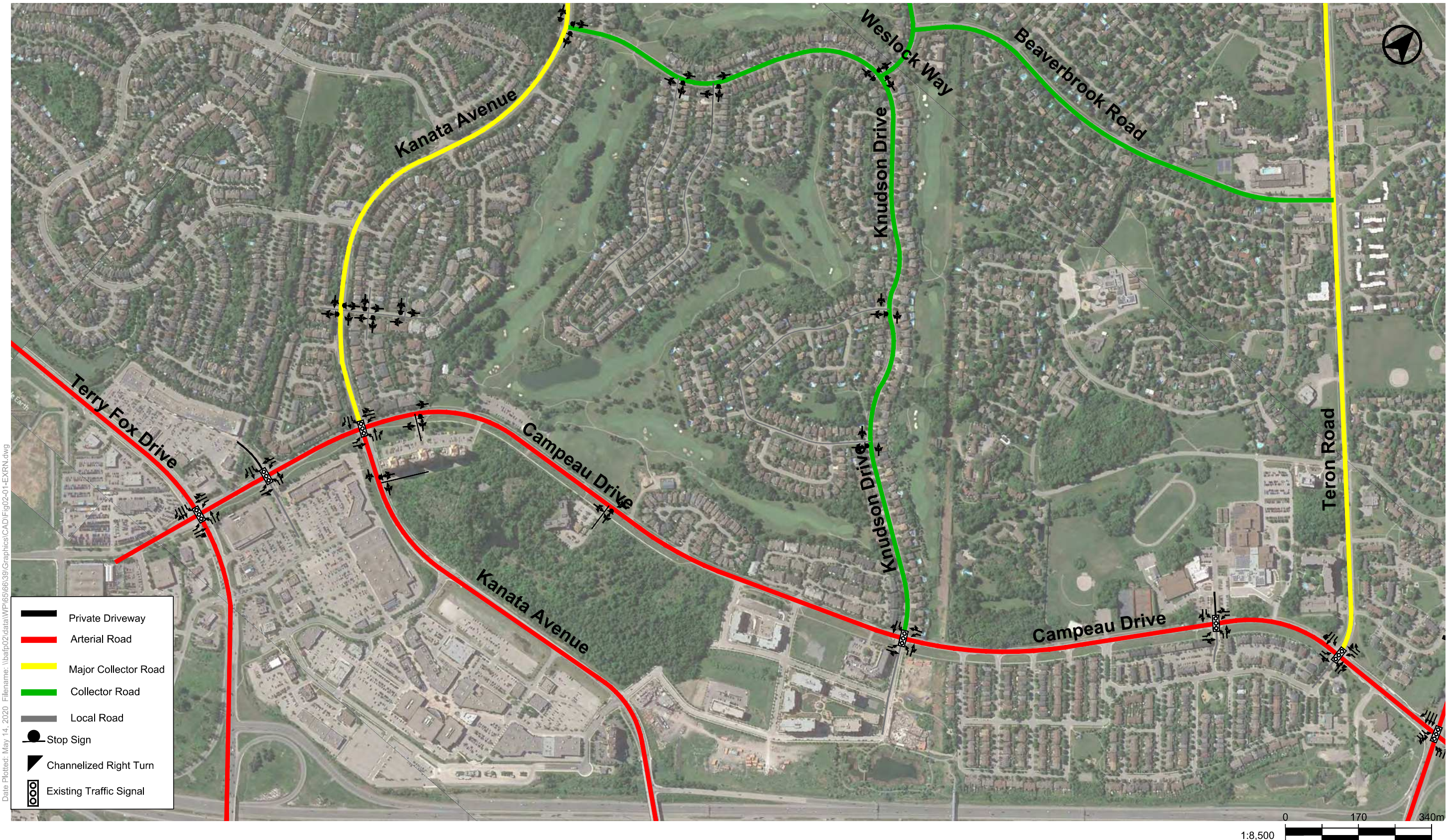
FIGURE 2 EXISTING ROAD NETWORK & LANE CONFIGURATIONS
