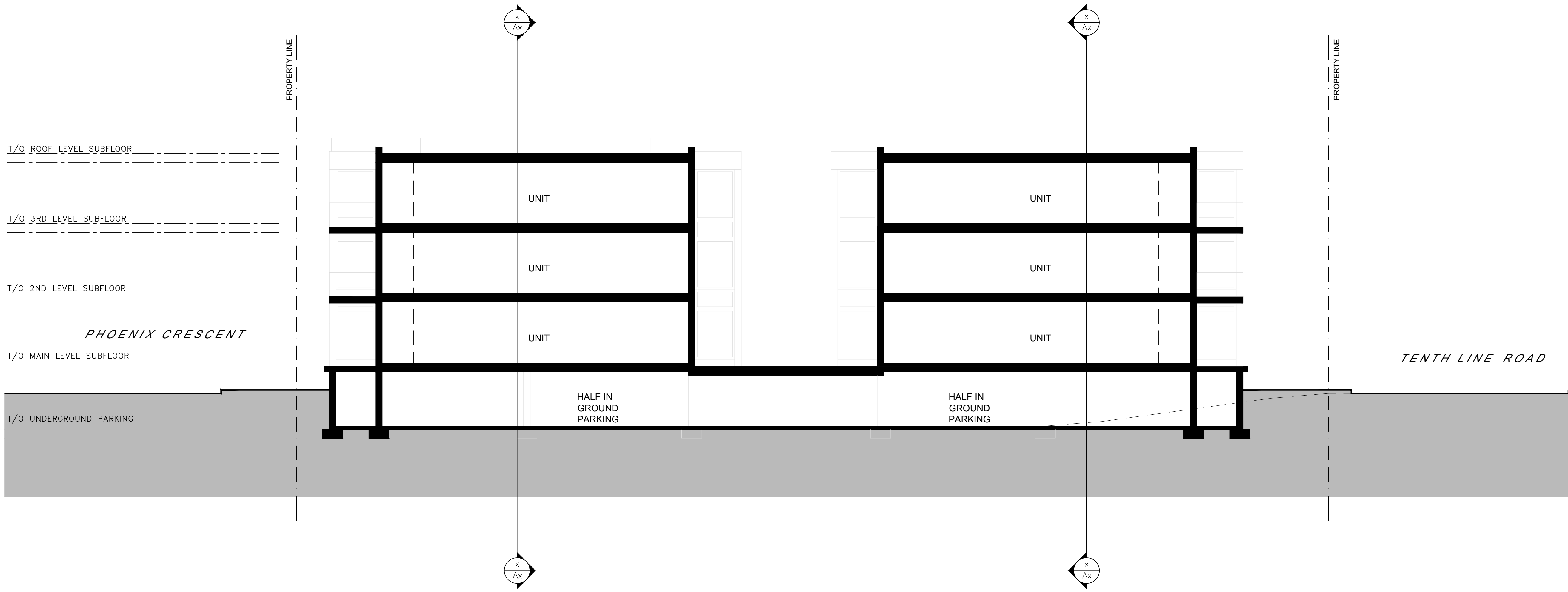
2 BUILDING SECTION A-300 SCALE = 1:100
