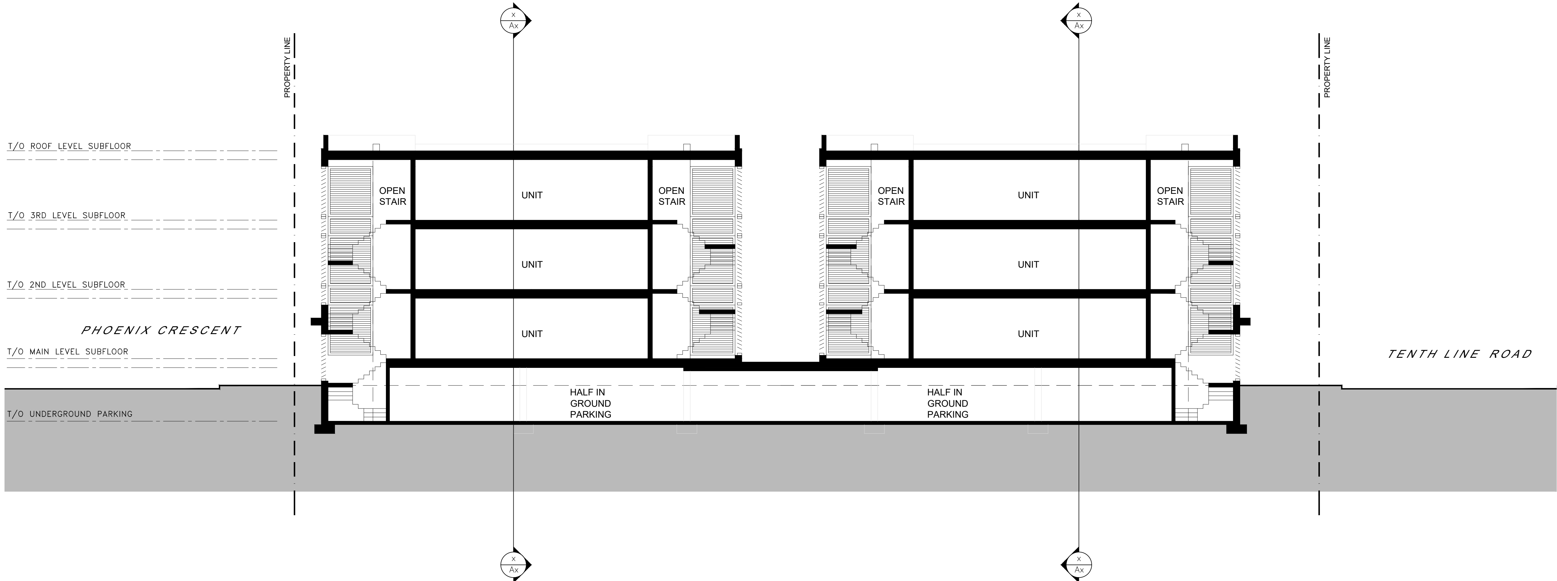
1 BUILDING SECTION (THROUGH OPEN STAIRS) A-300 SCALE = 1:100
