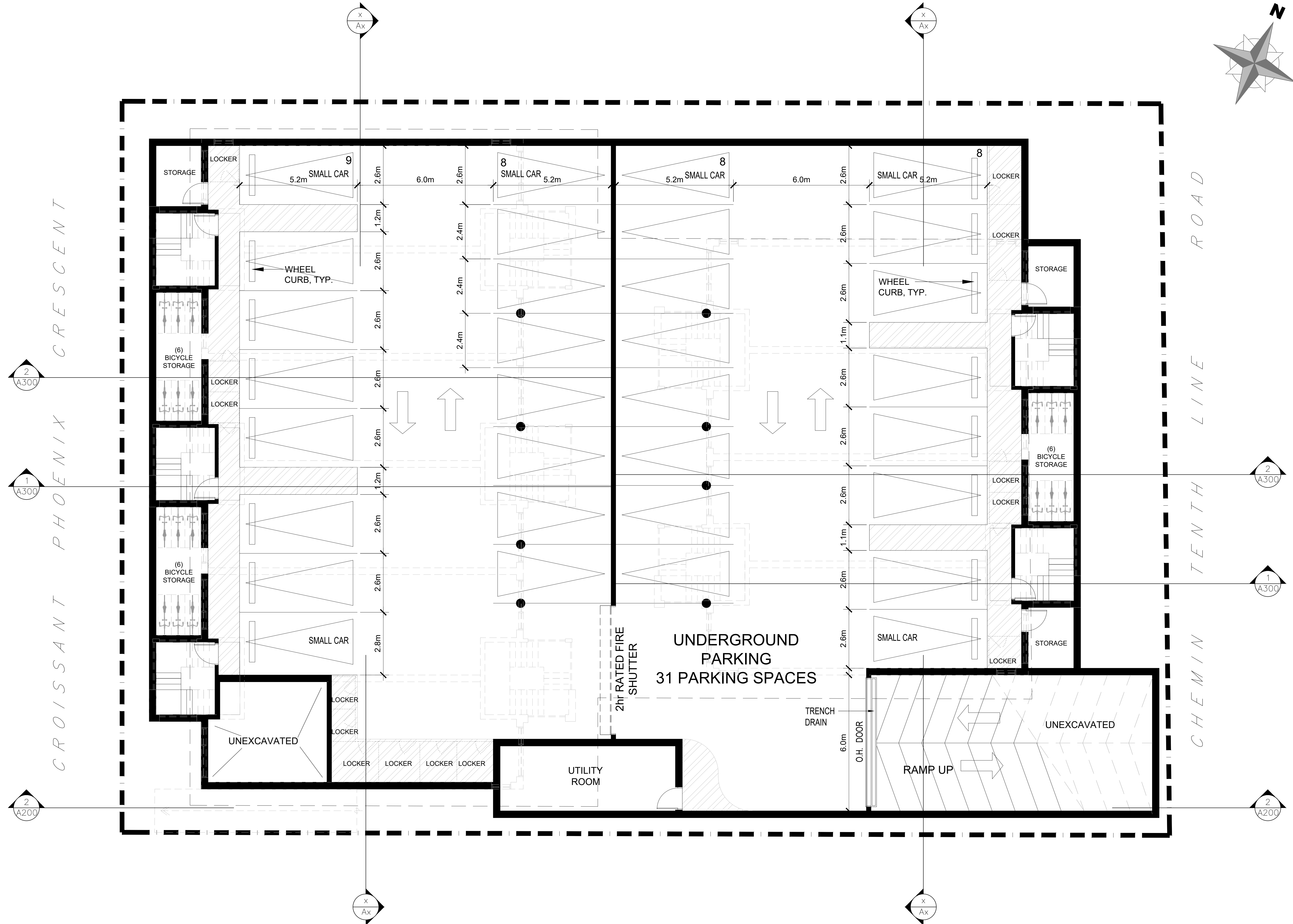
1 LOWER LEVEL FLOOR PLAN SCALE = 1:75
