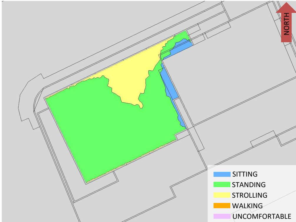
FIGURE 7C: AUTUMN – WIND COMFORT, LEVEL 7 COMMON AMENITY TERRACE
