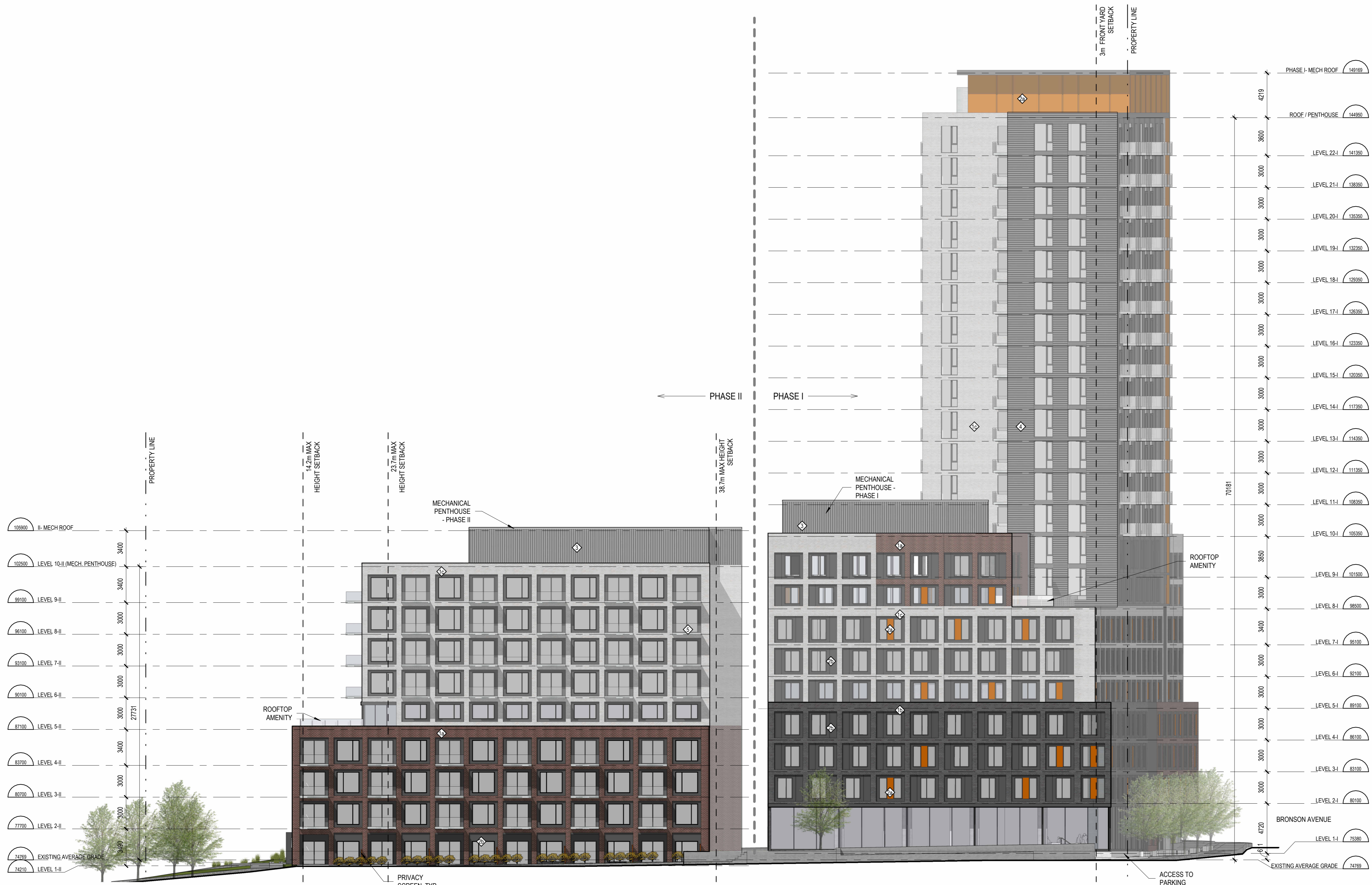
1 SOUTH ELEVATION A.203 1:200
