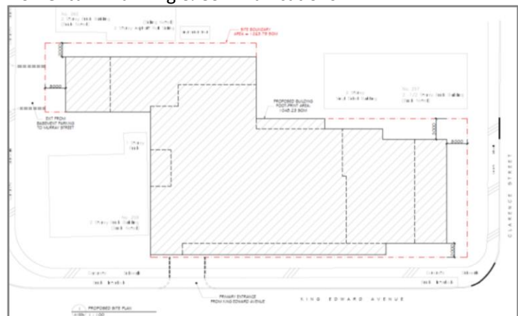
Figure 14: Bird’s Eye view and plan view showing the tightness and irregular shape. It was recommended that the property on the north-west side be purchased.
