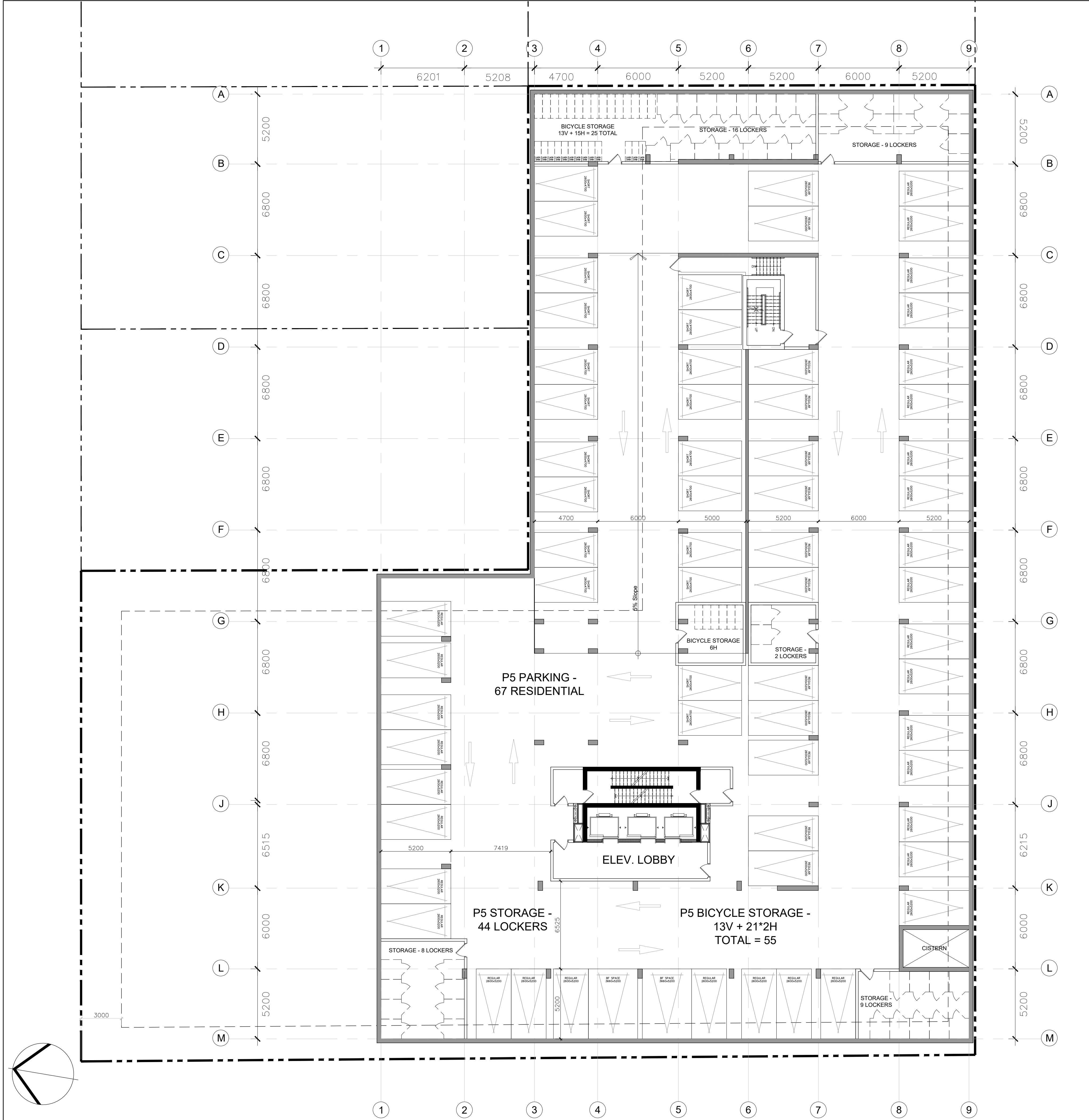
1 LEVEL P5 FLOOR PLAN A2.01 1:150
