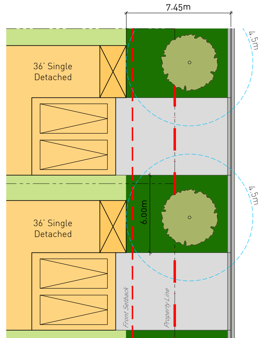
Alternating Driveways
