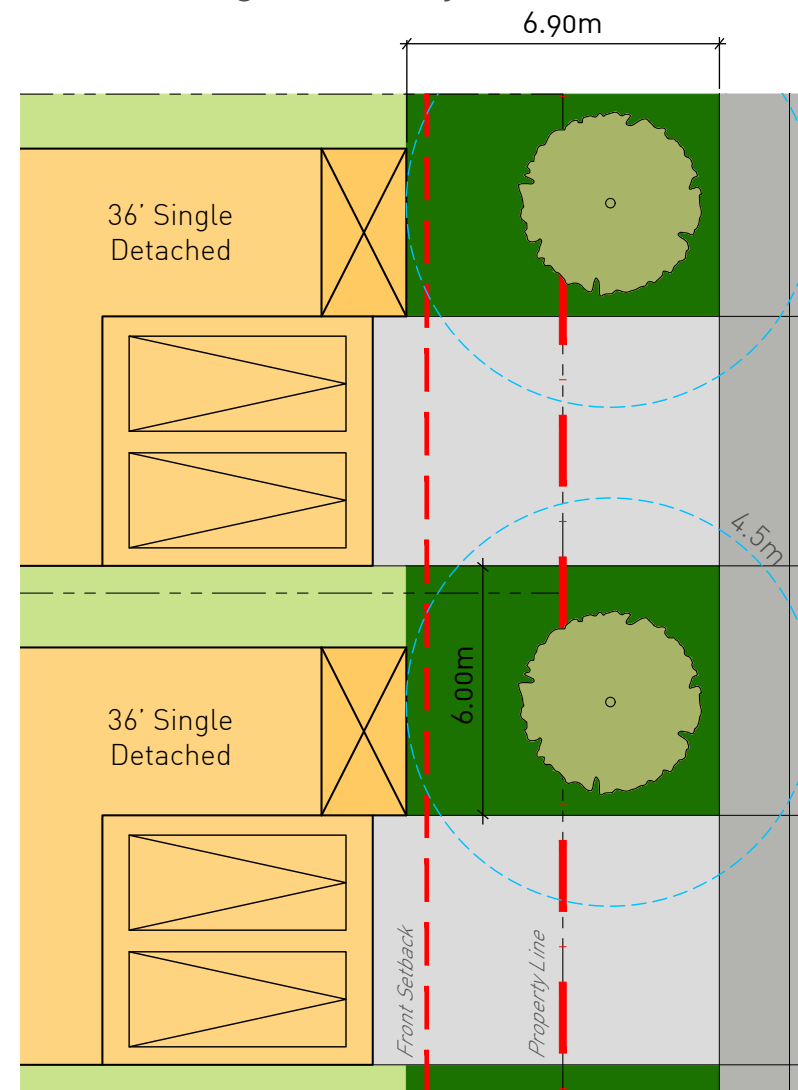
Alternating Driveways
