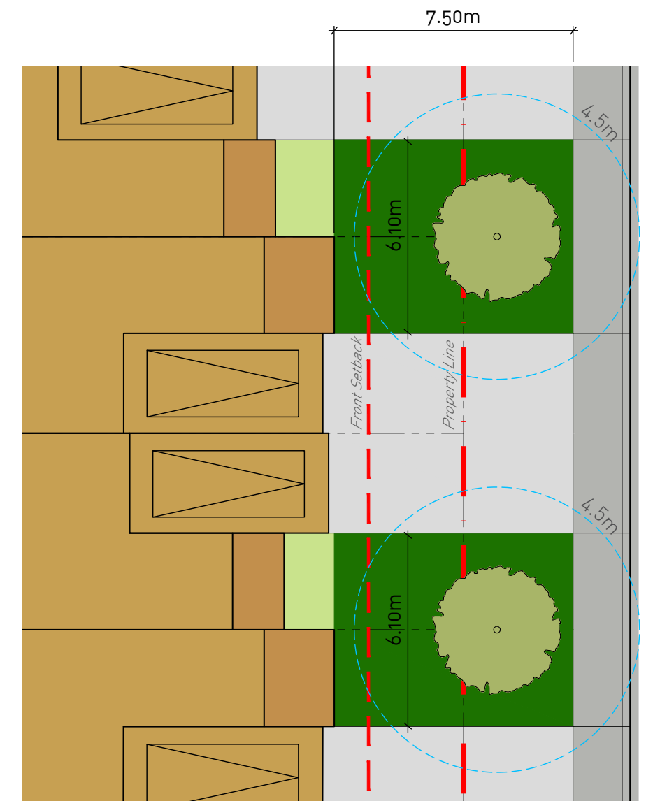
Street Townhouses
