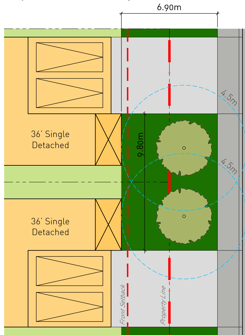
Separated Driveways
