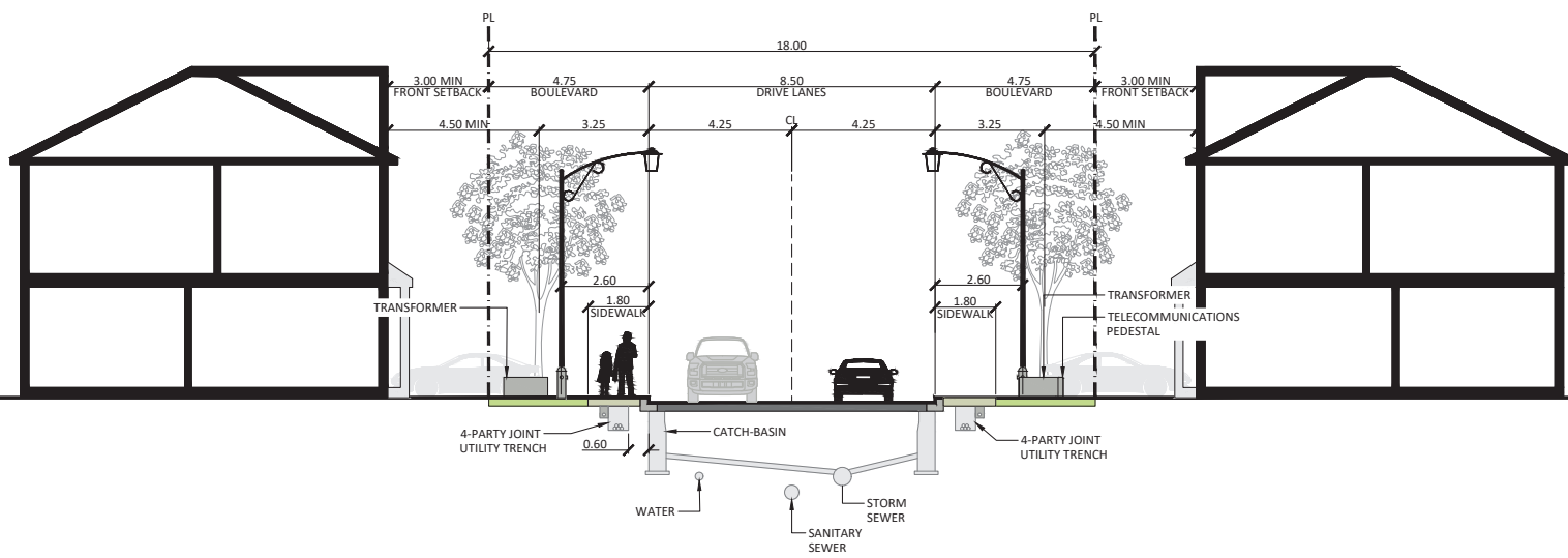
18.0m Local Road with Sidewalks
