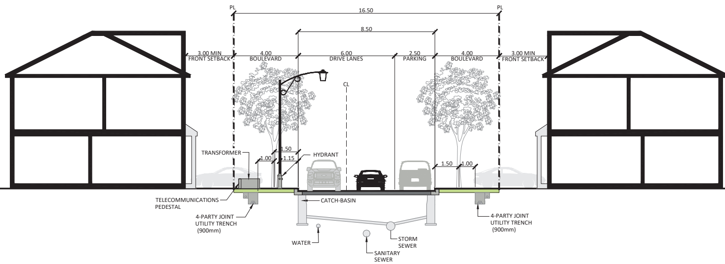
16.5m Local Road without Sidewalk
