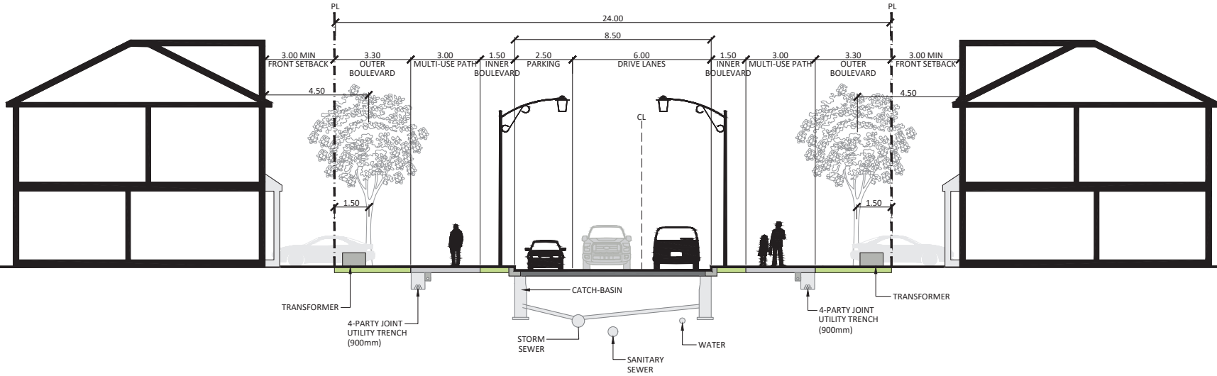
24.0m Collector with Multi-Use Path (MUP)
