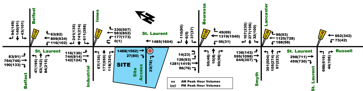
Figure 6: Existing Peak Hour Traffic Volumes
