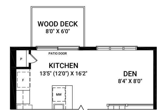
OPTIONAL PATIO DOOR WITH DECK
