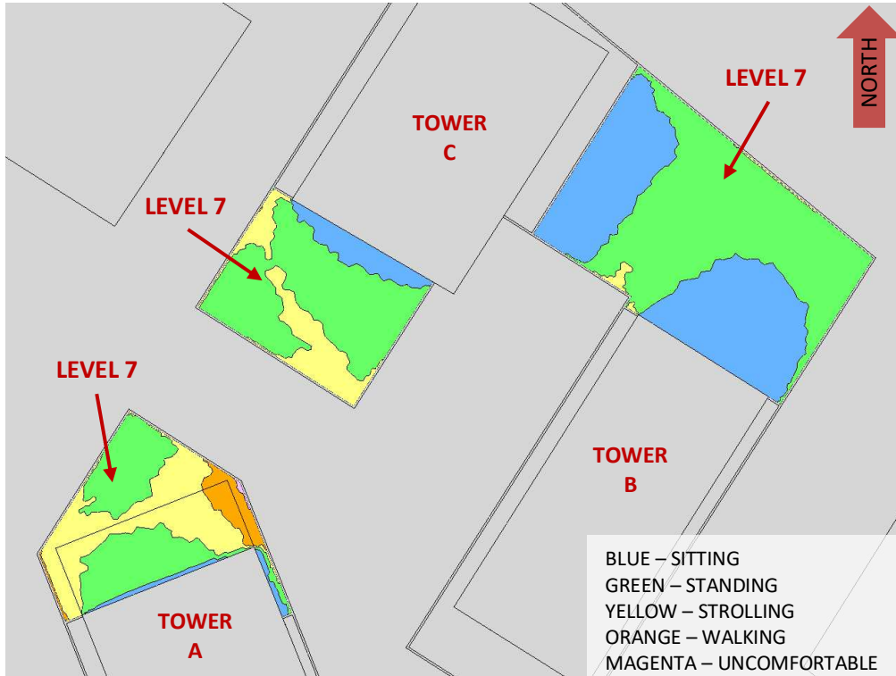
FIGURE 6A: TYPICAL USE PERIOD – WIND COMFORT, COMMON AMENITY TERRACES
