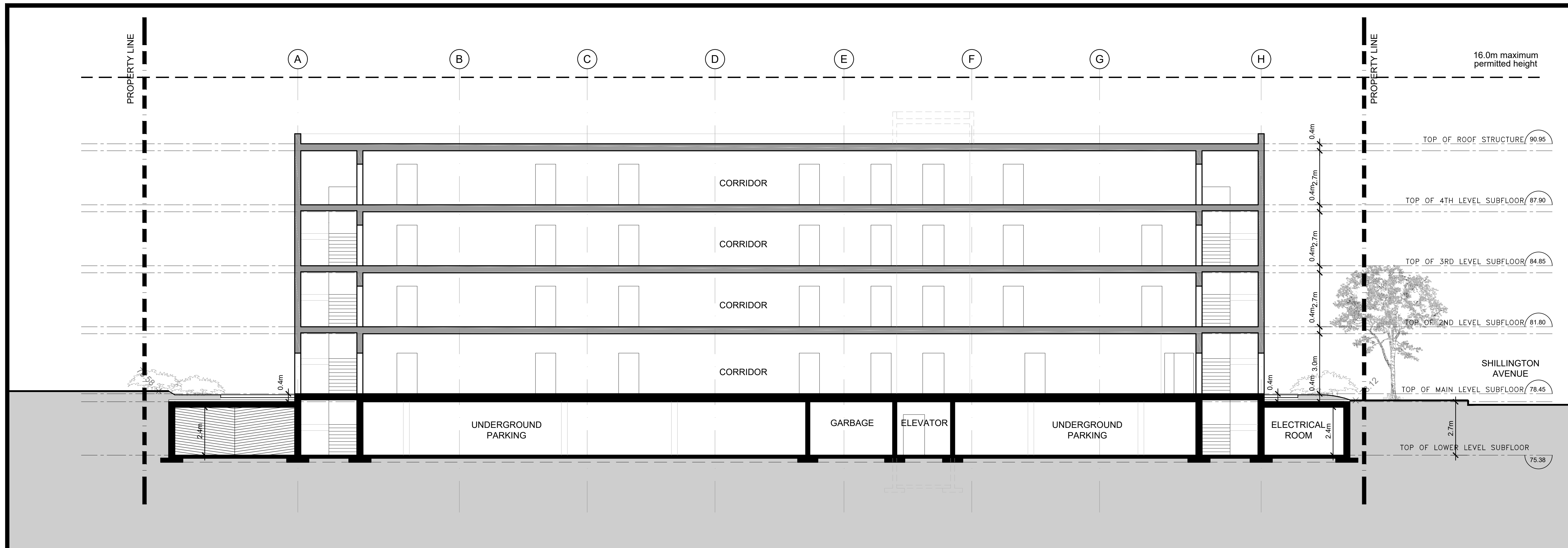
BUILDING SECTION
