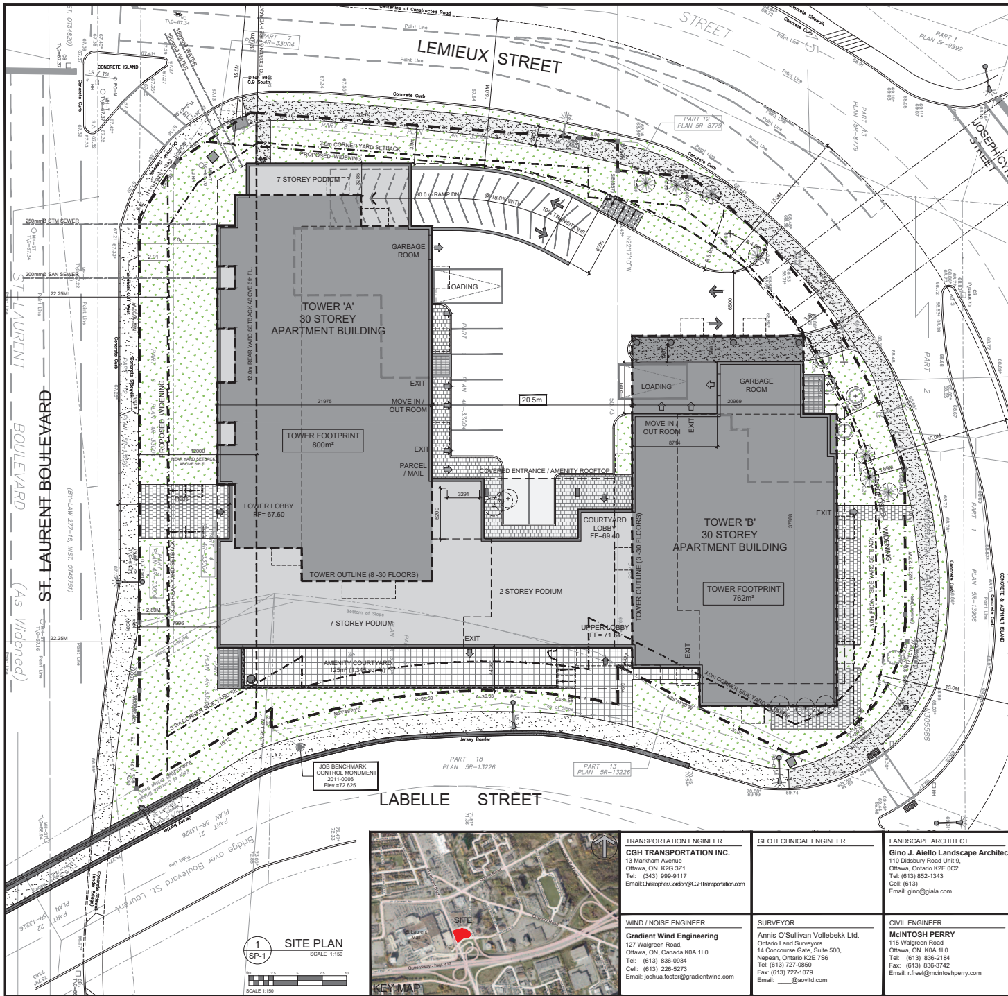
Figure 2: Concept Plan
