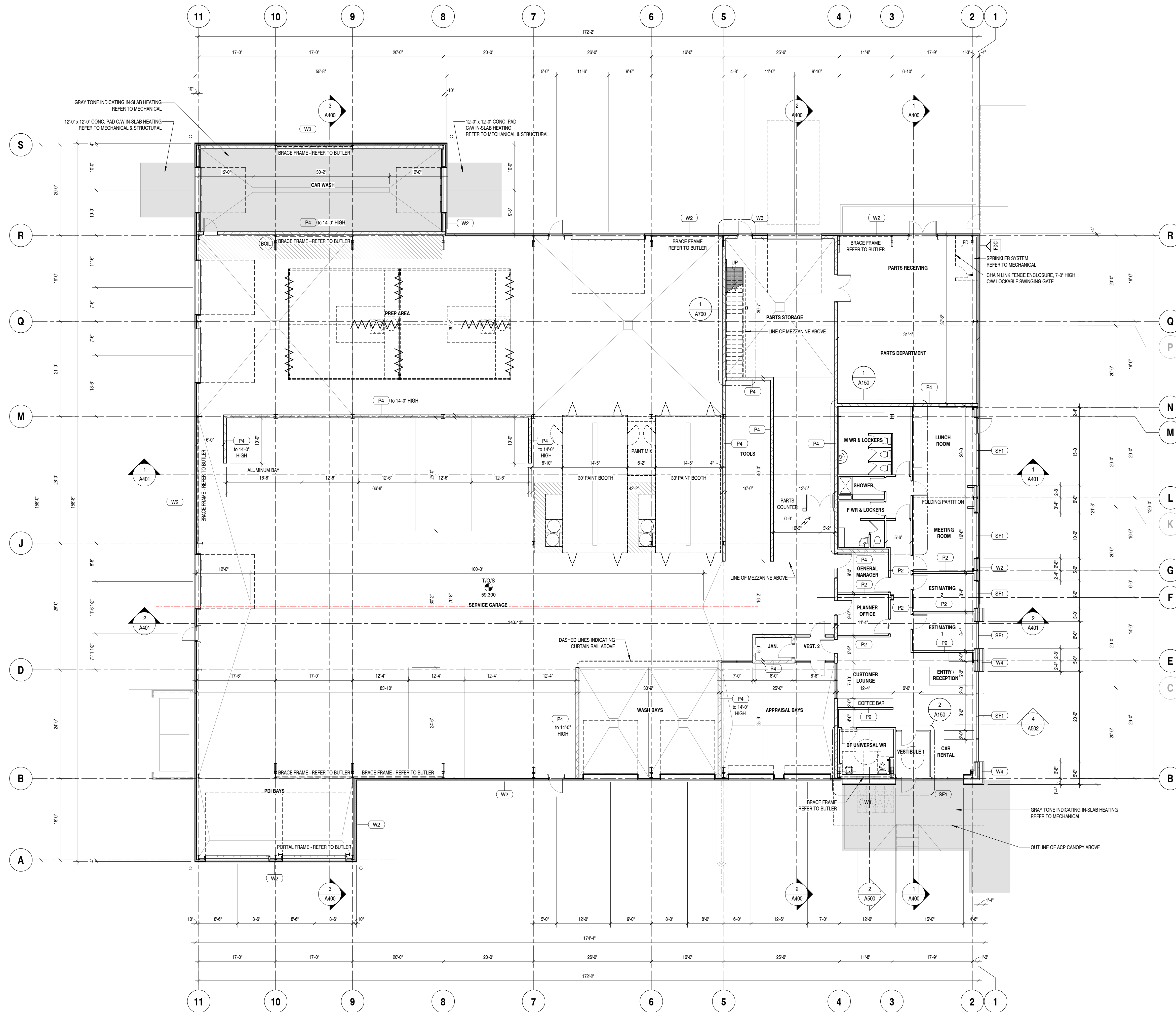
1 GROUND FLOOR PLAN A100 3/32" = 1'-0"
