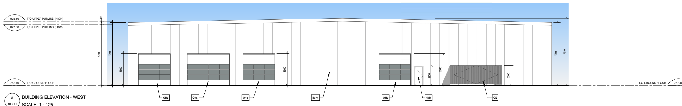
2 BUILDING ELEVATION - SOUTH A030 SCALE: 1 : 125
