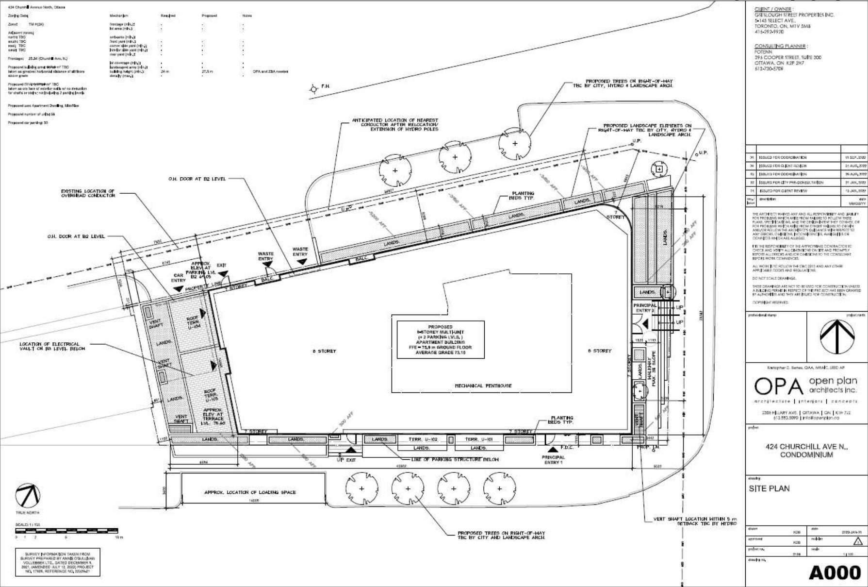
Exhibit 2-2: Site Plan (REV 04 2022)
