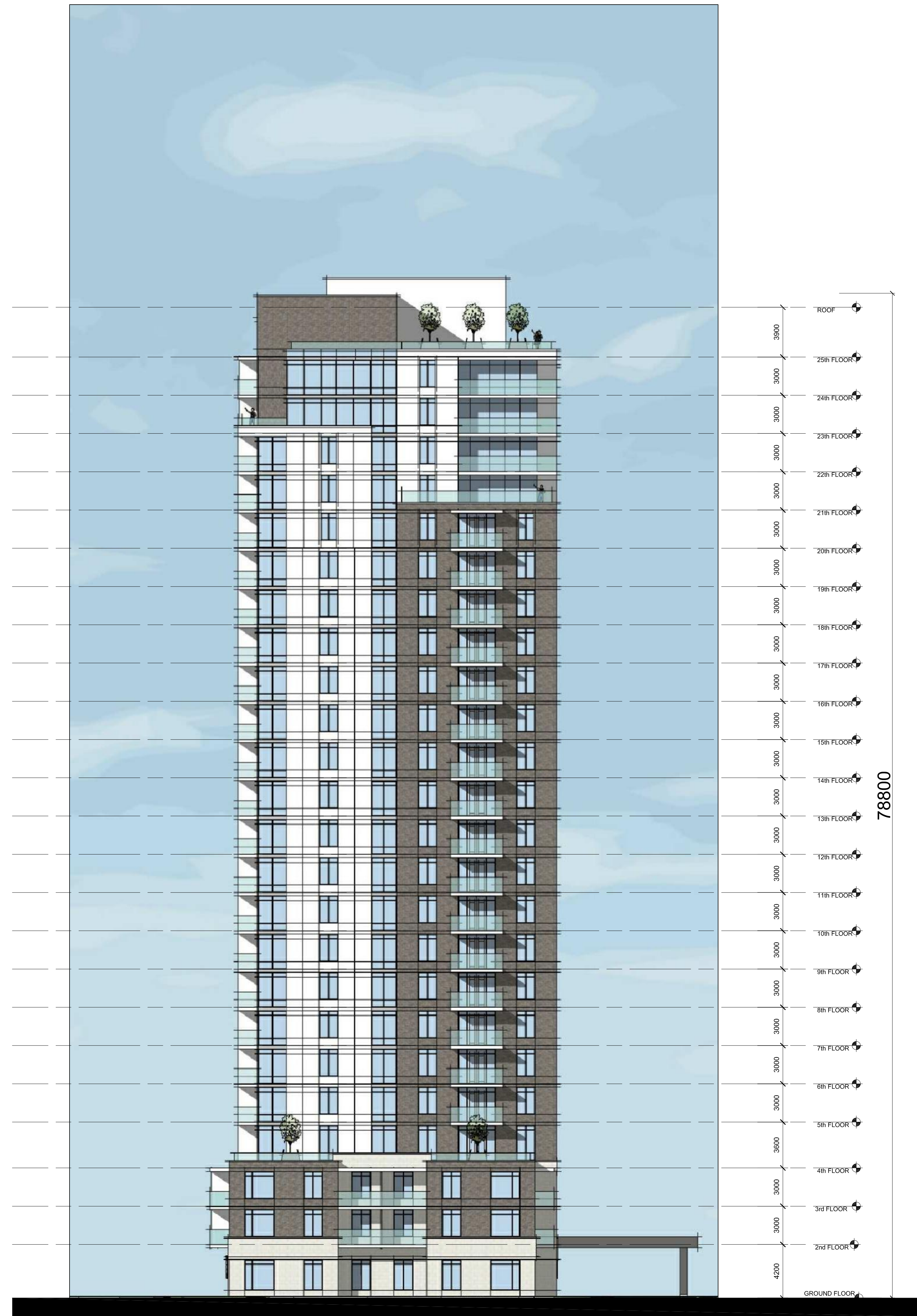
SOUTH ELEVATION
