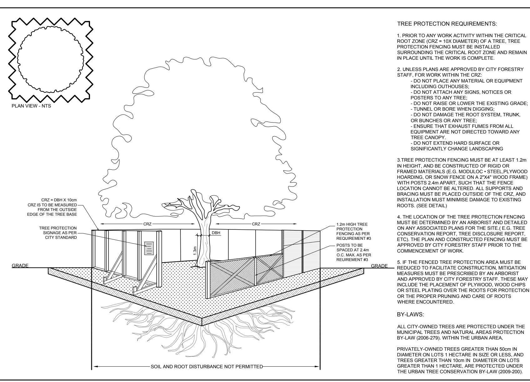
3 TREE PROTECTION FENCE SCALE: NTS
