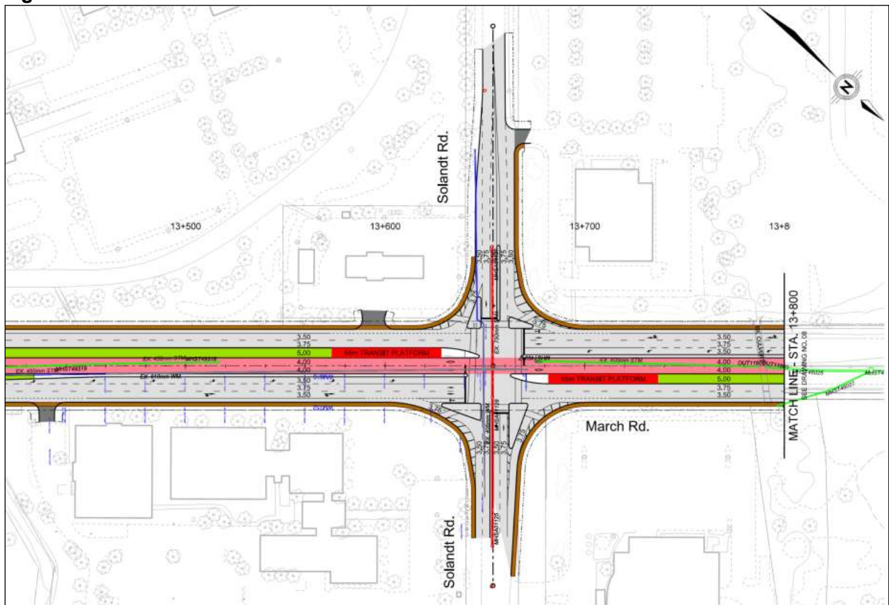
Figure 14: Planned Modifications to March Road/Solandt Road
