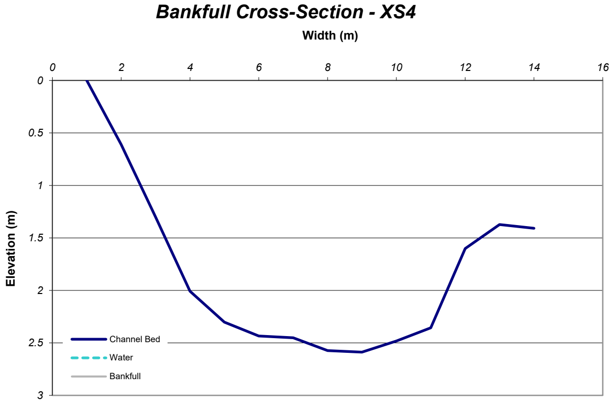
FIGURE B5 Cross-section profile at XS4 from tops of slope, right to left facing downstream
