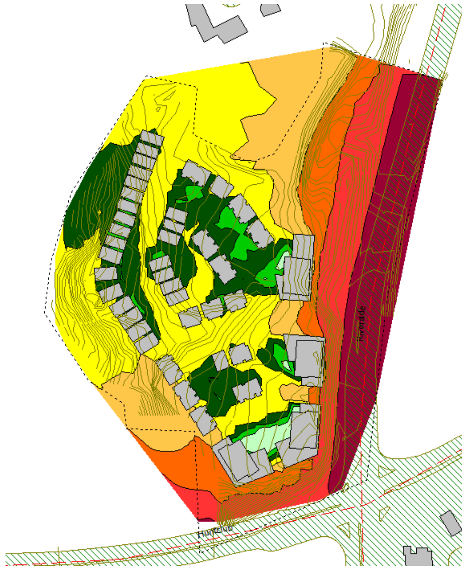
FIGURE 8: NIGHTTIME TRAFFIC NOISE CONTOURS, WITH MID-RISE (4.5 M ABOVE GRADE)
