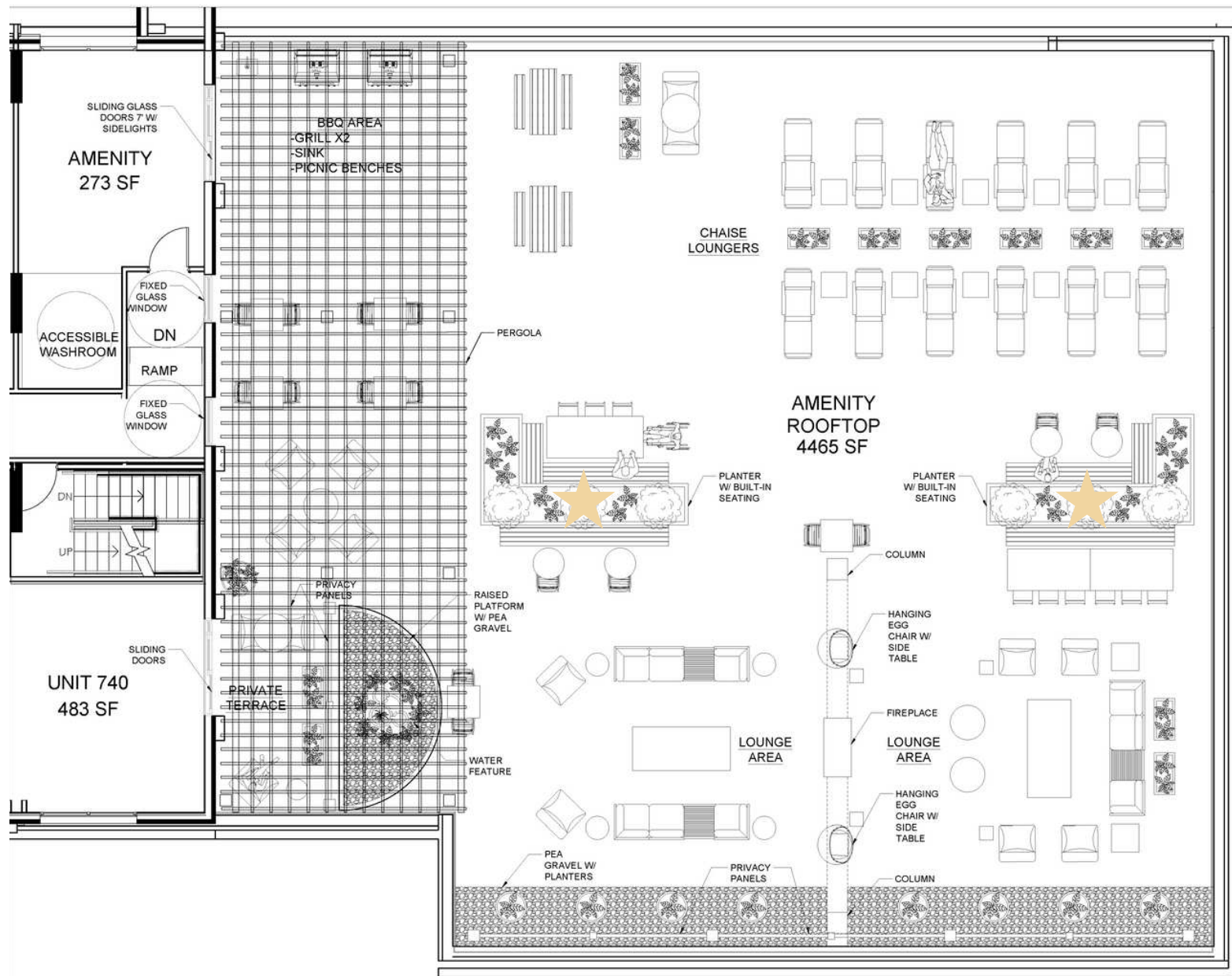
SP08 7 th FLOOR - PROPOSED ROOFTOP SPACE PLAN (PERGOLA) 112 NELSON ST
