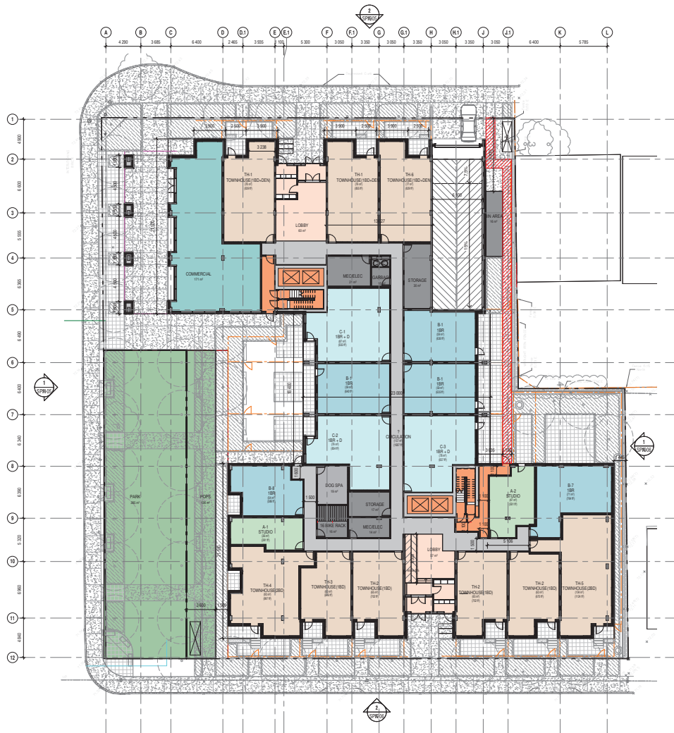
GROUND FLOOR 1:200
