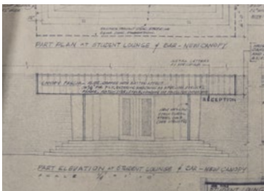
Figure 6. Canopy elevation (Murray & Murray, 1974) and photo of front entry canopy (ERA, 2021).
