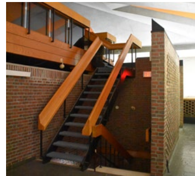
Figure 4. Building A Section (Murray & Murray, 1974) and photo of stair to mezzanine (ERA, 2021).
