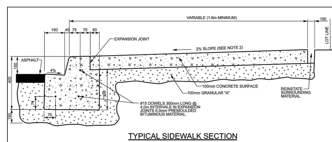
TYPICAL SIDEWALK SECTION
