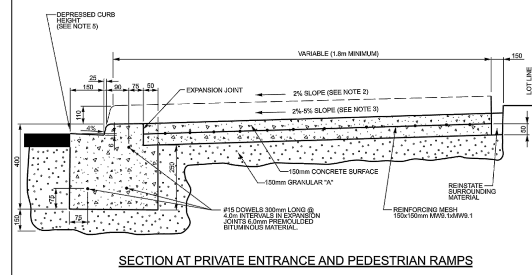
SECTION AT PRIVATE ENTRANCE AND PEDESTRIAN RAMPS
