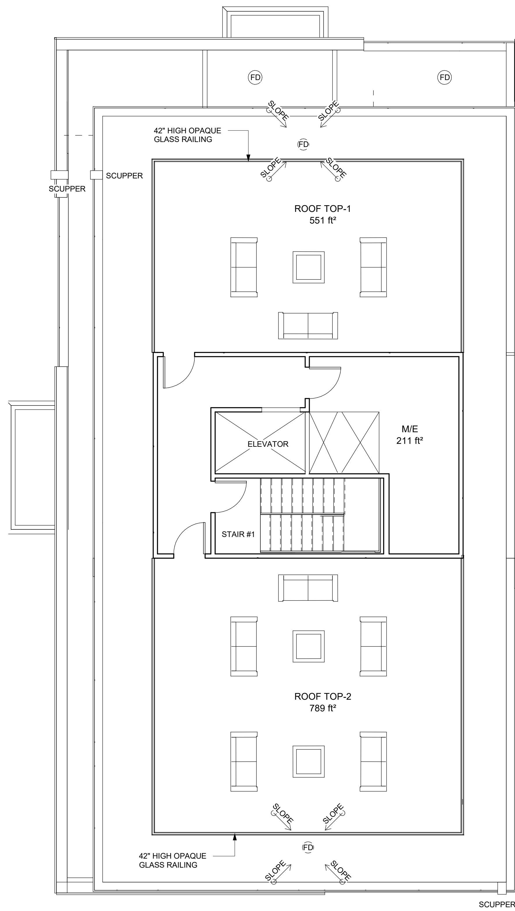
1 Roof 1:75
