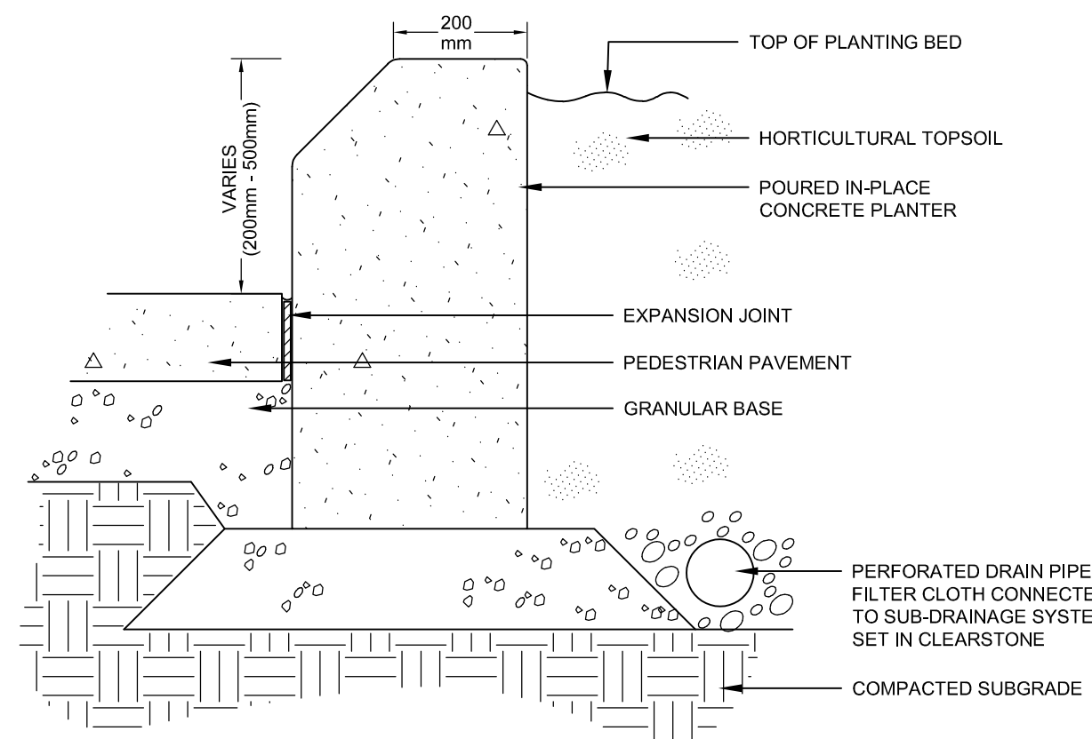
2 CURB-STYLE PLANTER
