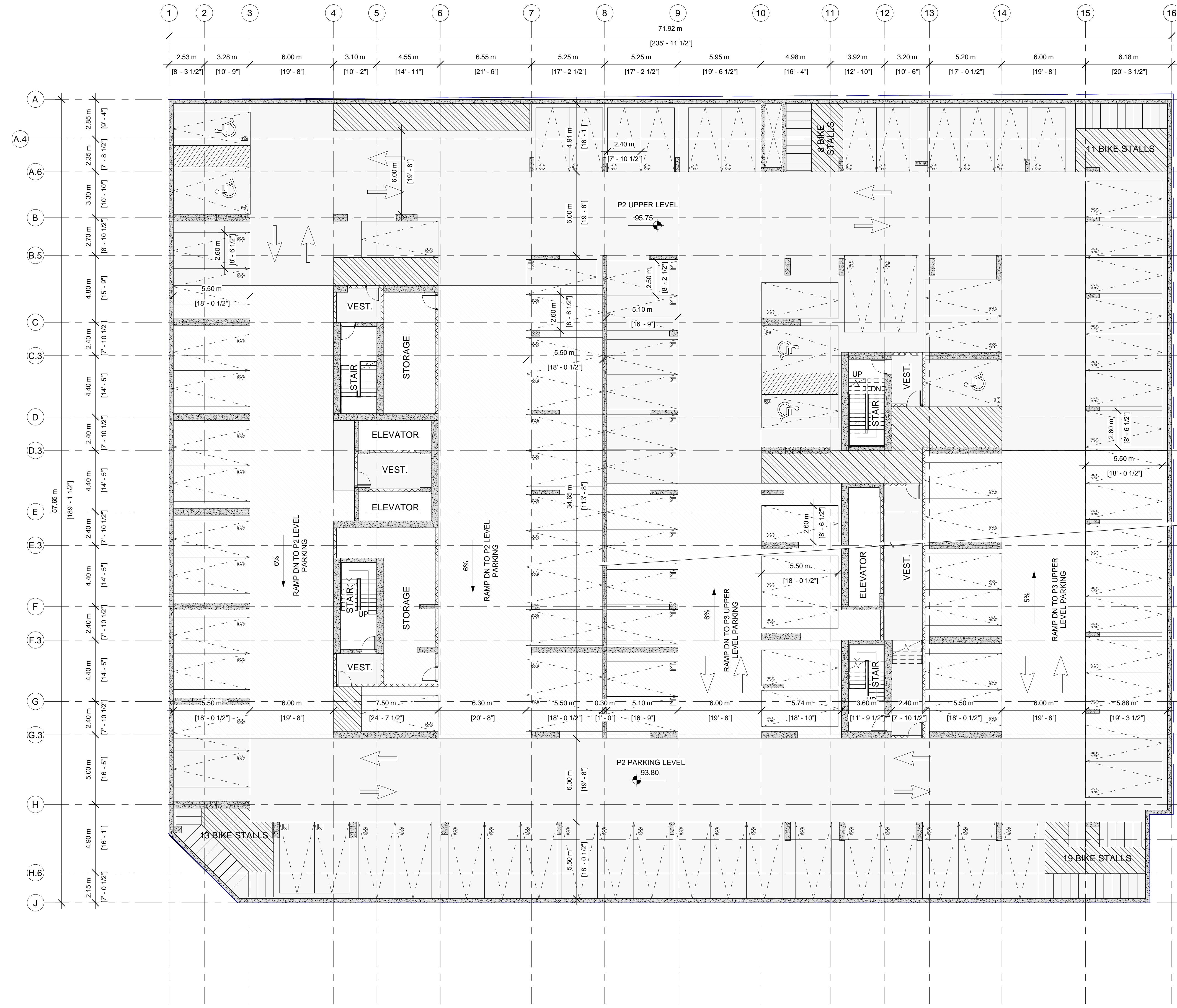
1 P2- P6 TYPICAL PARKING PLANS 1 : 150
