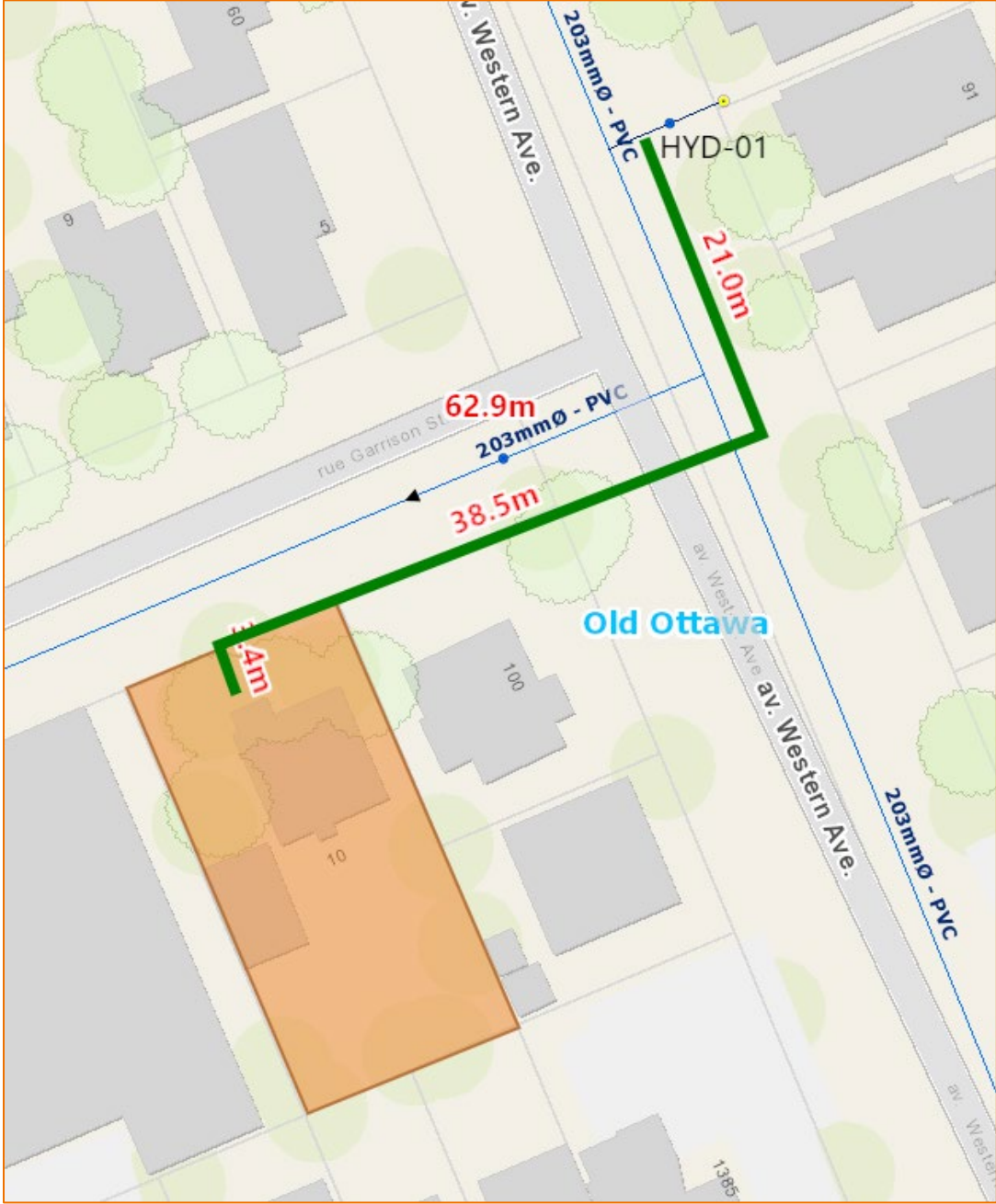
Figure 3.1: Existing Fire Hydrant Coverage Map
