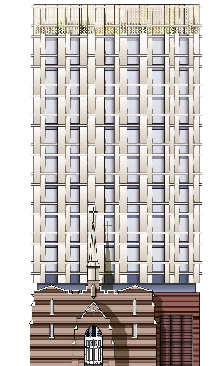
NORTH ELEVATION
