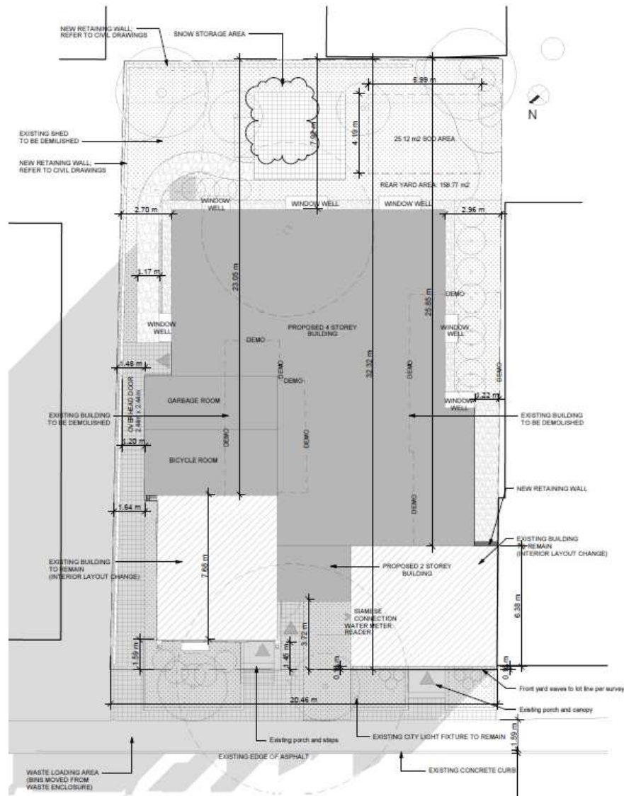
Figure 7: Site Plan of Proposed Development
