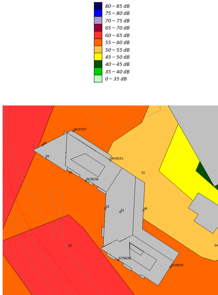
FIGURE 4: NIGHTTIME NOISE CONTOURS (4.5M ABOVE GRADE)
