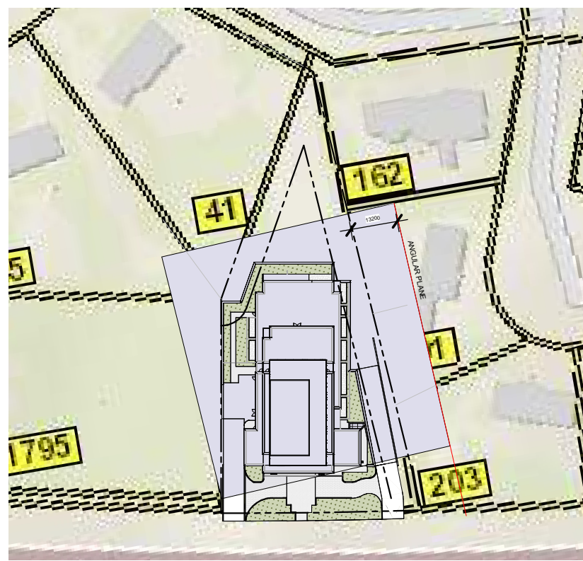
EAST SIDE ANGULAR PLAN OPTION 1
