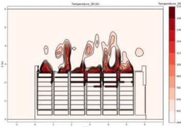
Figure 4-12: Top front corner ignition temperature map (outside).
