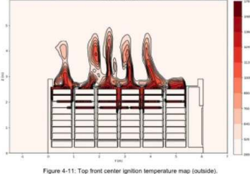
Figure 4-11: Top front center ignition temperature map (outside).
