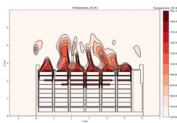
Figure 4-10: Top center ignition temperature map (outside).
