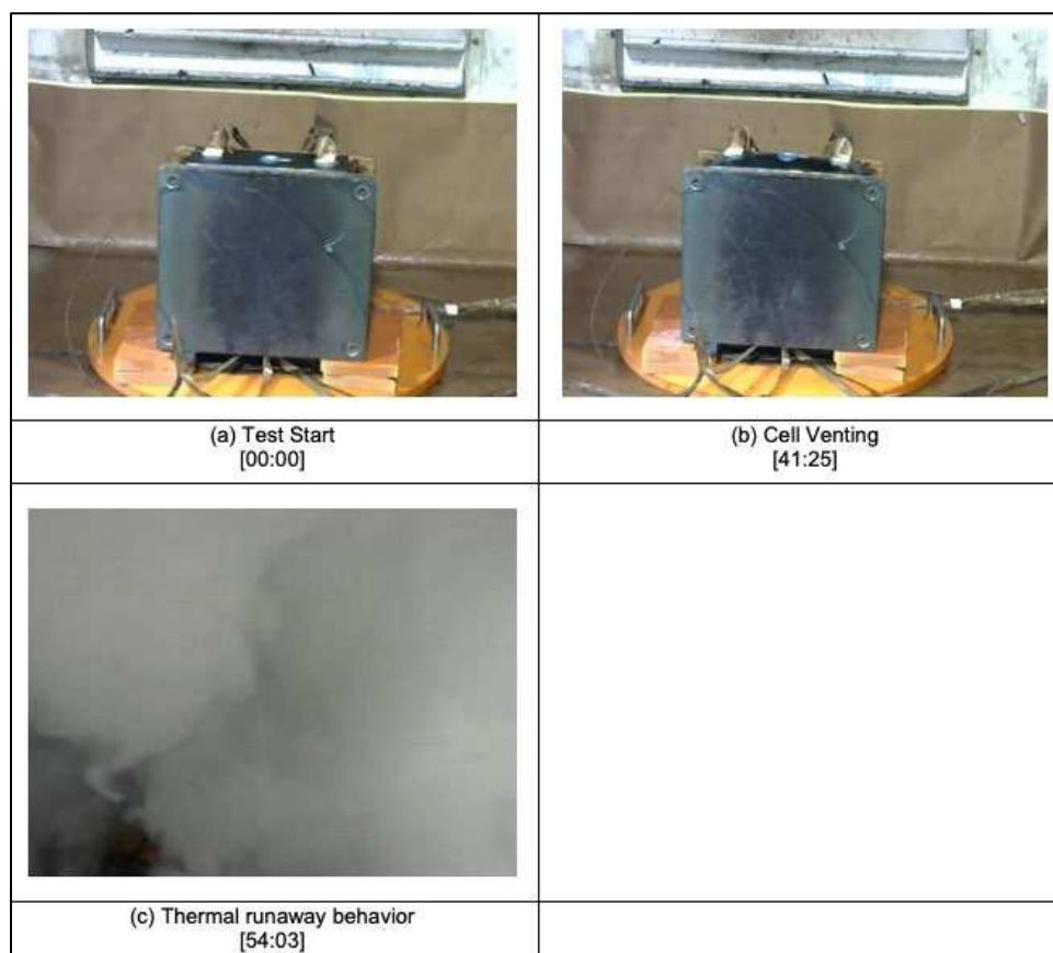
Figure 9 – Highlights of Cell 1 Testing
