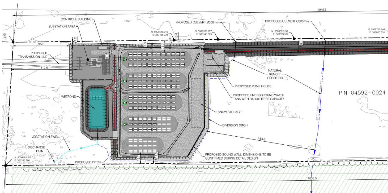
Figure 2. Site Plan Excerpt (BBA, dated 2025-05-13)
