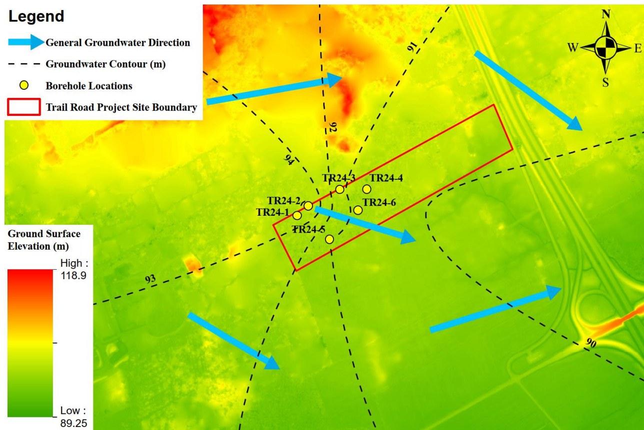
Figure 2-3: General Groundwater Flow Directions
