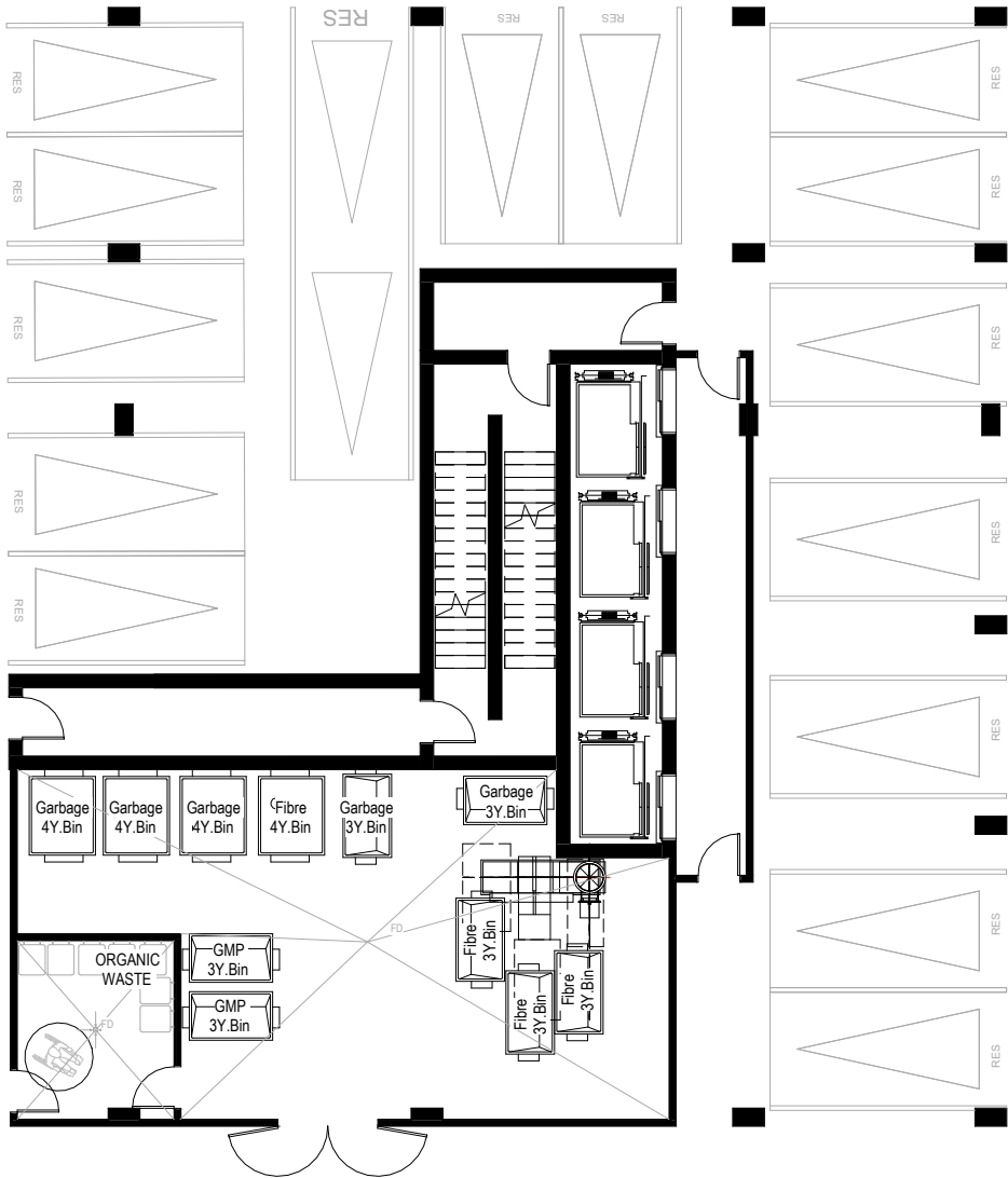
GARBAGE ROOM BUILDING 3
