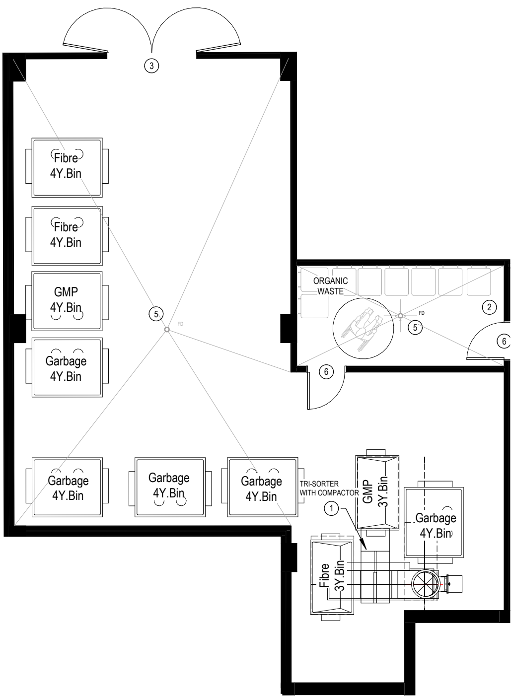
GARBAGE ROOM BUILDING 2 ENLARGED
